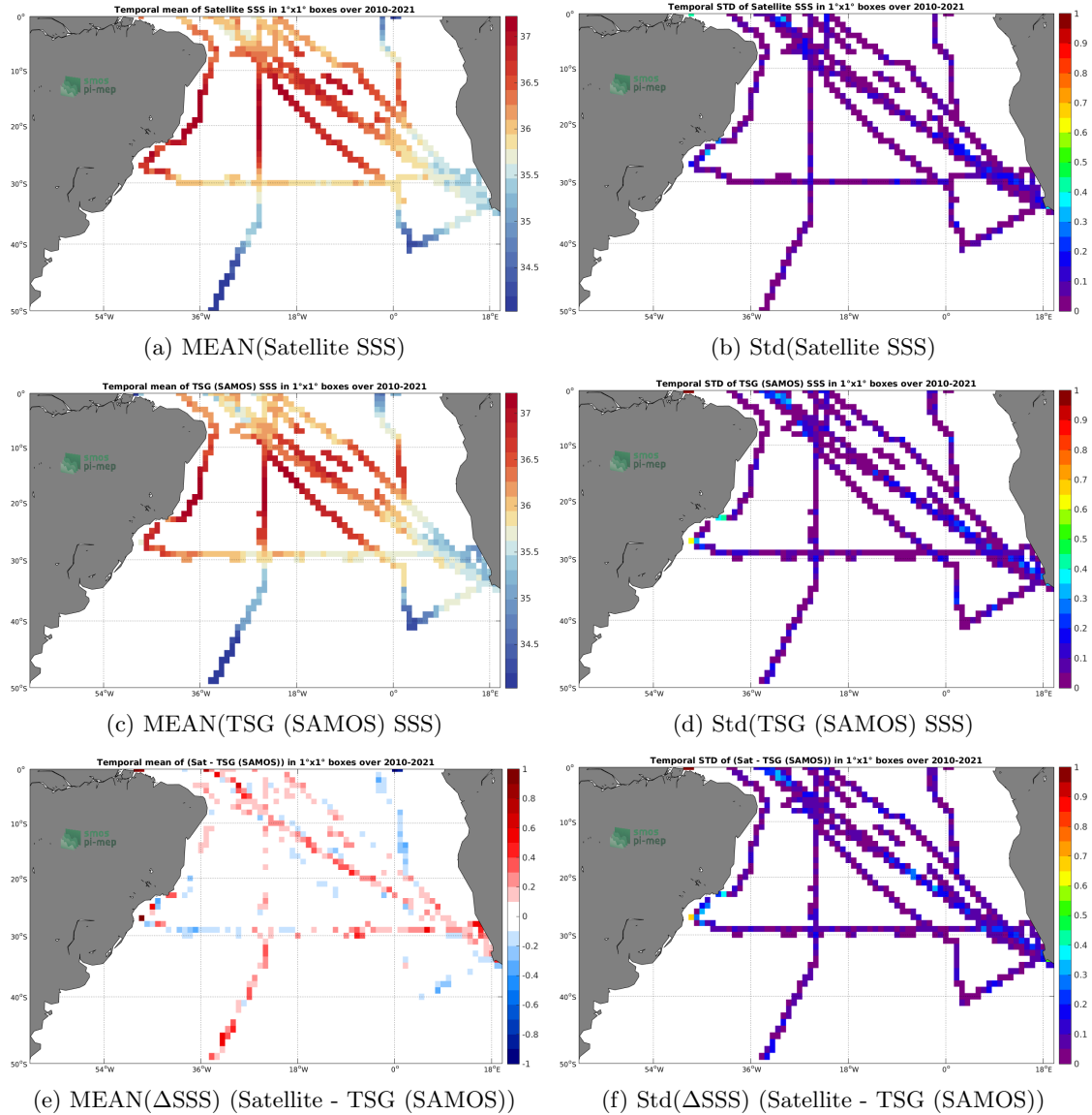
Figure 6: Temporal mean (left) and Std (right) of SSS from SMOS SSS L3 v7 - 18 Days (CATDS-CECOS-LOCEAN) (top), TSG (SAMOS) (middle), and of \Delta SSS (Satellite - TSG (SAMOS)). Only match-up pairs are used to generate these maps.
