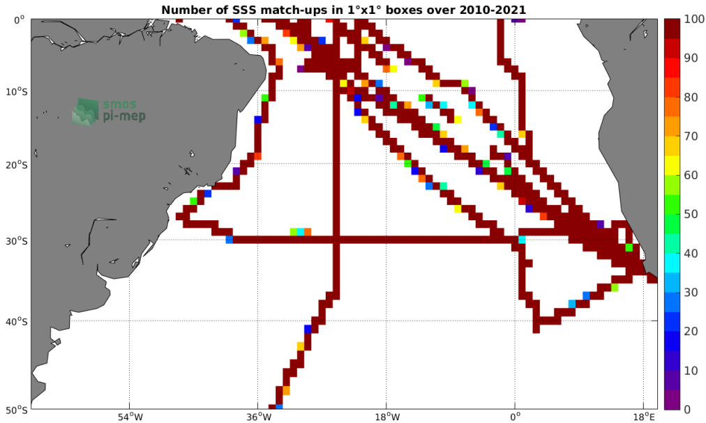
Figure 4: Number of SSS match-ups between TSG (SAMOS) SSS and the SMOS SSS L3 v7 - 18 Days (CATDS-CECOS-LOCEAN) SSS product for the South Atlantic Ocean Pi-MEP region over 1^{\circ} \times 1^{\circ} boxes and for the full satellite product period.
