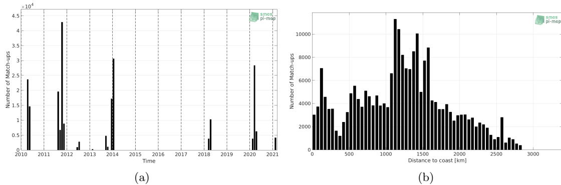
Figure 1: Number of match-ups between TSG (SAMOS) and SMOS SSS L3 v7 - 18 Days (CATDS-CECOS-LOCEAN) SSS as a function of time (a) and as function of the distance to coast (b) over the South Atlantic Ocean Pi-MEP region and for the full satellite product period.
