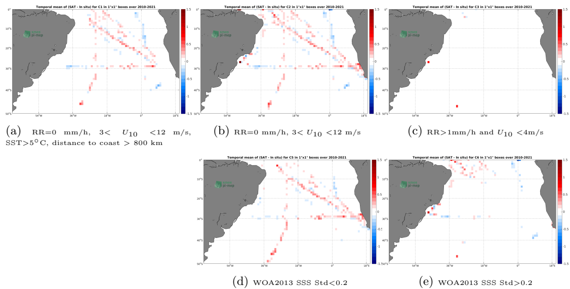
Figure 12: Temporal mean gridded over spatial boxes of size 1^\circ \times 1^\circ of \Delta SSS (SMOS SSS L3 v7 - 18 Days (CATDS-CECOS-LOCEAN) - TSG (SAMOS)) for 5 different subdatasets corresponding to: RR=0 mm/h, 3 < U_{10} < 12 m/s, SST > 5^\circ\text{C} , distance to coast > 800 km (a), RR=0 mm/h, 3 < U_{10} < 12 m/s (b), RR > 1 mm/h and U_{10} < 4 m/s (c), WOA2013 SSS Std < 0.2 (d), WOA2013 SSS Std > 0.2 (e).
