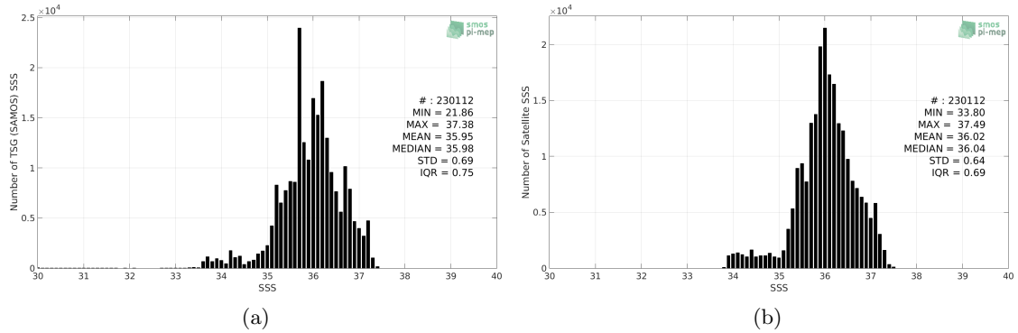
Figure 2: Histograms of SSS from TSG (SAMOS) (a) and SMOS SSS L3 v7 - 18 Days (CATDS-CECOS-LOCEAN) (b) considering all match-up pairs per bins of 0.1 over the South Atlantic Ocean Pi-MEP region and for the full satellite product period.
