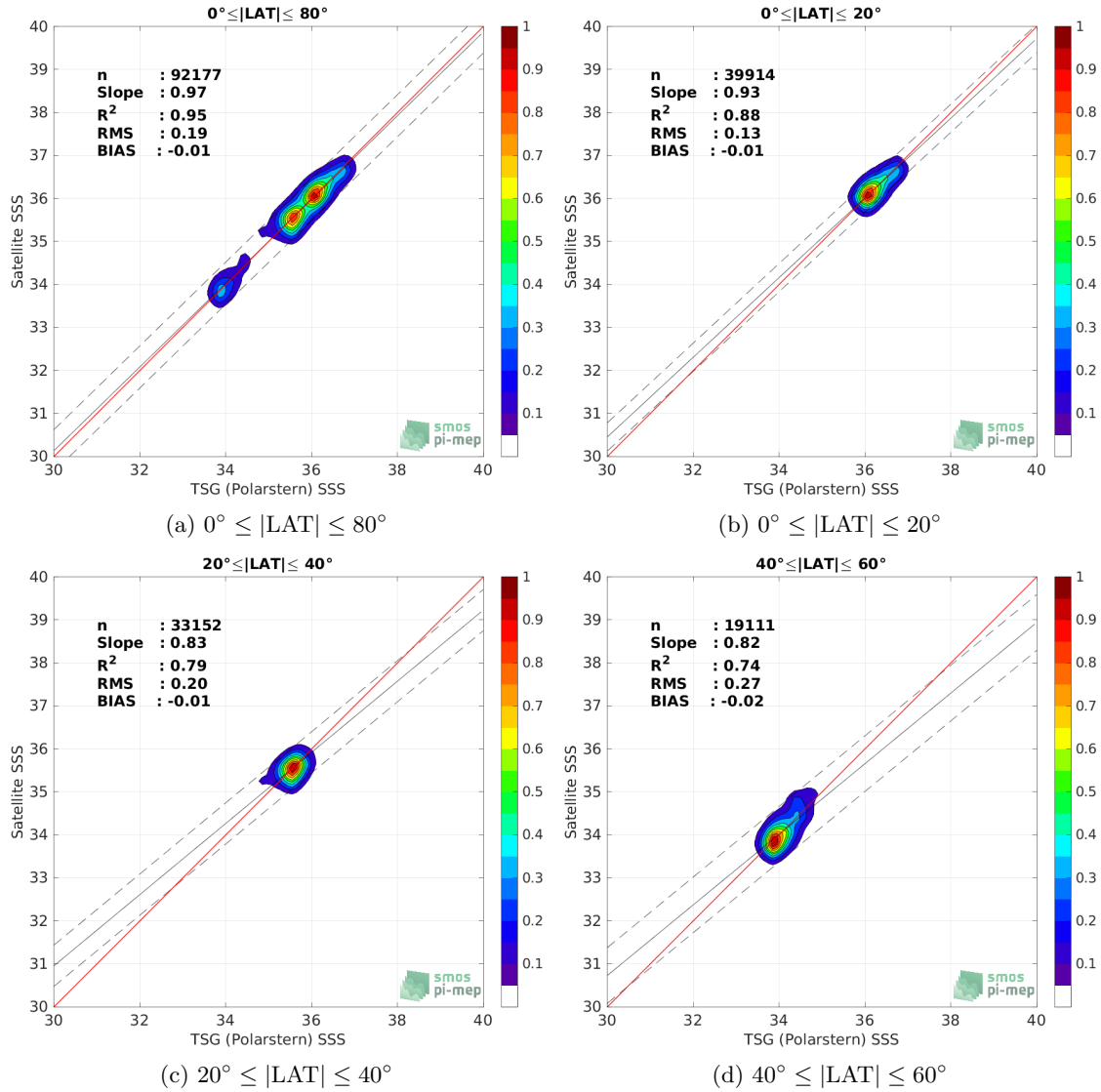
Figure 9: Contour maps of the concentration of SMOS SSS L3 v7 - 18 Days (CATDS-CECOS-LOCEAN) SSS ( y -axis) versus TSG (Polarstern) SSS ( x -axis) at match-up pairs for different latitude bands. For each plot, the red line shows x=y . The black thin and dashed lines indicate a linear fit through the data cloud and the \pm 95\% confidence levels, respectively. The number match-up pairs n , the slope and R^2 coefficient of the linear fit, the root mean square (RMS) and the mean bias between satellite and in situ data are indicated for each latitude band in each plots.
