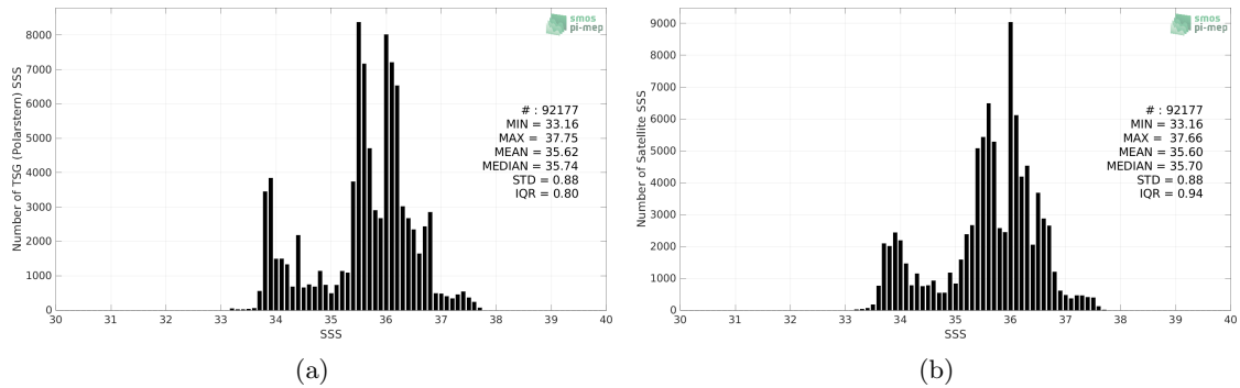
Figure 2: Histograms of SSS from TSG (Polarstern) (a) and SMOS SSS L3 v7 - 18 Days (CATDS-CECOS-LOCEAN) (b) considering all match-up pairs per bins of 0.1 over the South Atlantic Ocean Pi-MEP region and for the full satellite product period.
