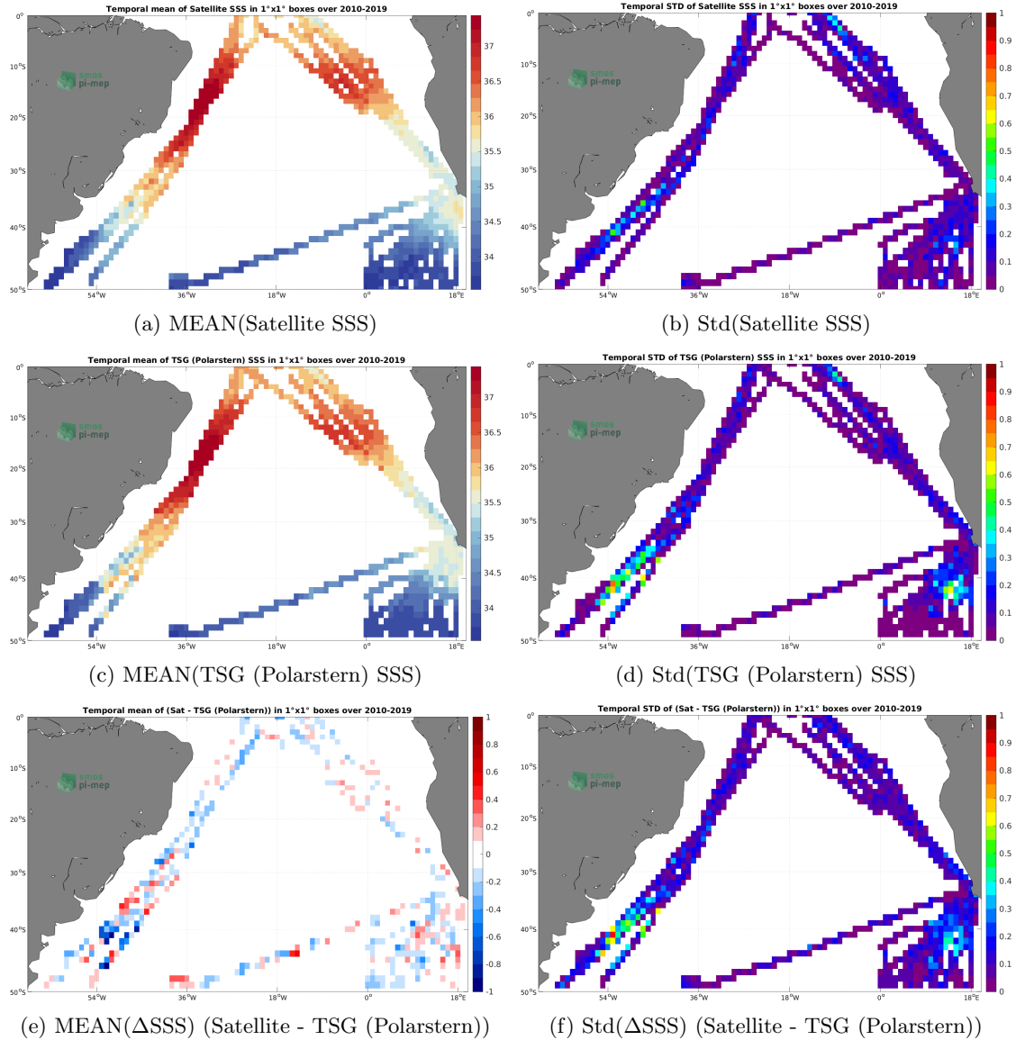
Figure 6: Temporal mean (left) and Std (right) of SSS from SMOS SSS L3 v7 - 18 Days (CATDS-CECOS-LOCEAN) (top), TSG (Polarstern) (middle), and of \Delta SSS (Satellite - TSG (Polarstern)). Only match-up pairs are used to generate these maps.
