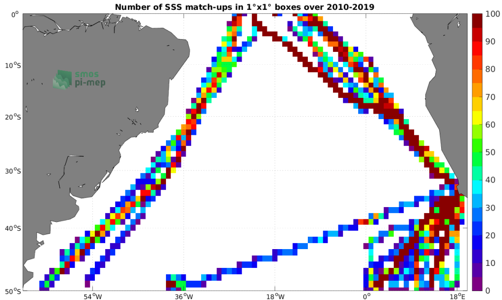
Figure 4: Number of SSS match-ups between TSG (Polarstern) SSS and the SMOS SSS L3 v7 - 18 Days (CATDS-CECOS-LOCEAN) SSS product for the South Atlantic Ocean Pi-MEP region over 1^\circ \times 1^\circ boxes and for the full satellite product period.
