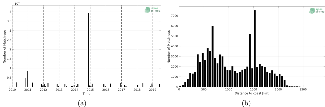
Figure 1: Number of match-ups between TSG (Polarstern) and SMOS SSS L3 v7 - 18 Days (CATDS-CECOS-LOCEAN) SSS as a function of time (a) and as function of the distance to coast (b) over the South Atlantic Ocean Pi-MEP region and for the full satellite product period.
