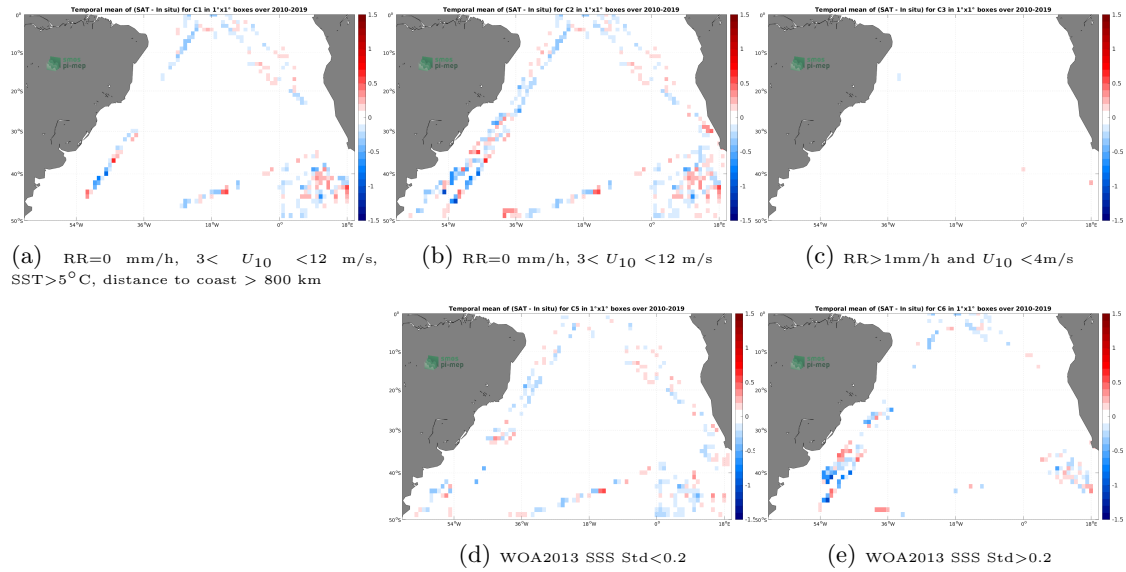
Figure 12: Temporal mean gridded over spatial boxes of size 1^\circ \times 1^\circ of \Delta\text{SSS} (SMOS SSS L3 v7 - 18 Days (CATDS-CECOS-LOCEAN) - TSG (Polarstern)) for 5 different subdatasets corresponding to:RR=0 mm/h, 3 < U_{10} < 12 m/s, SST >5^\circ\text{C} , distance to coast > 800 km (a), RR=0 mm/h, 3 < U_{10} < 12 m/s (b), RR >1 mm/h and U_{10} < 4 m/s (c), WOA2013 SSS Std <0.2 (d), WOA2013 SSS Std >0.2 (e).
