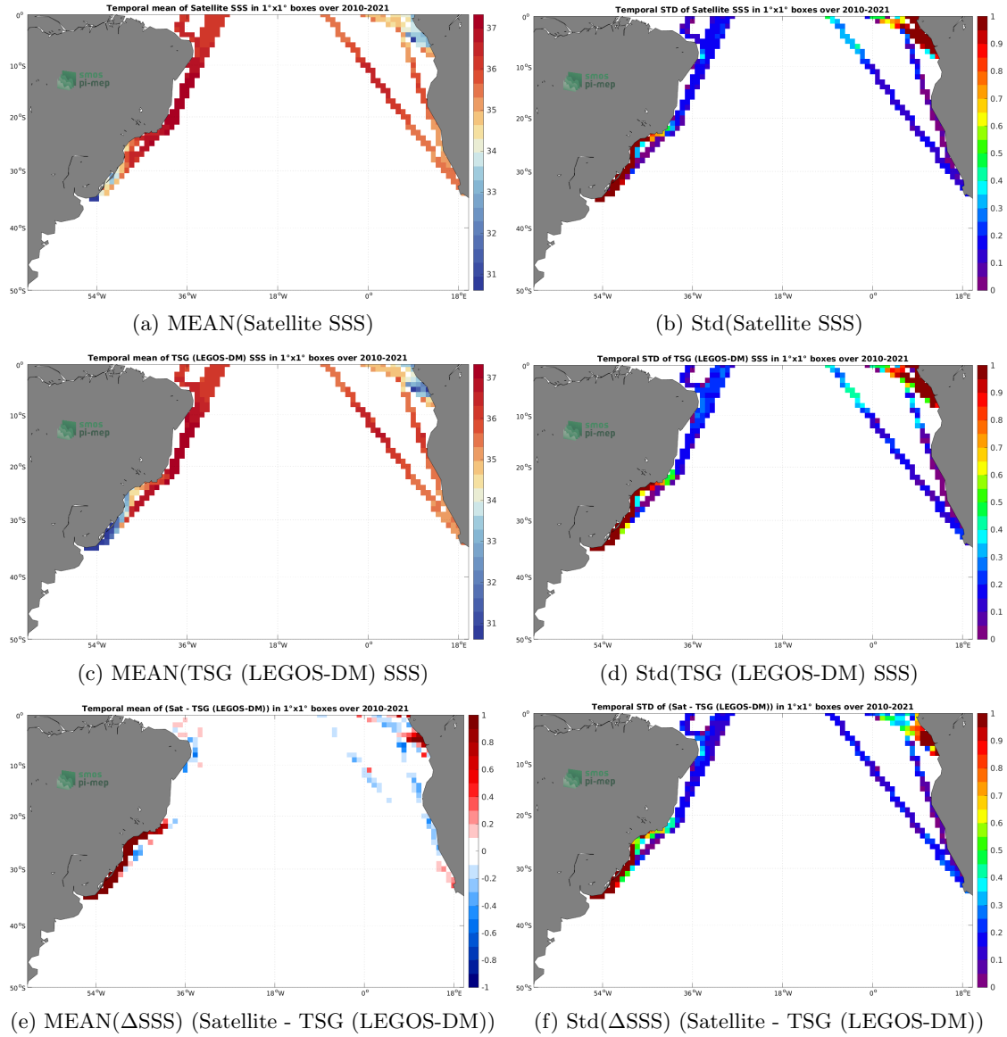
Figure 6: Temporal mean (left) and Std (right) of SSS from SMOS SSS L3 v7 - 18 Days (CATDS-CECOS-LOCEAN) (top), TSG (LEGOS-DM) ( in situ ) dataset (middle), and of \Delta SSS (Satellite - TSG (LEGOS-DM)). Only match-up pairs are used to generate these maps.
