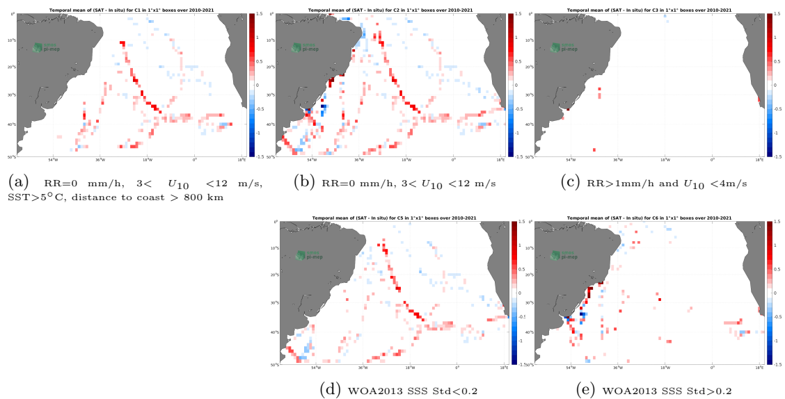
Figure 12: Temporal mean gridded over spatial boxes of size 1^\circ \times 1^\circ of \Delta\text{SSS} (SMOS SSS L3 v7 - 18 Days (CATDS-CECOS-LOCEAN) - TSG (GOSUD-Sailing-ship)) for 5 different subdatasets corresponding to:RR=0 mm/h, 3 < U_{10} < 12 m/s, SST >5^\circ\text{C} , distance to coast > 800 km (a), RR=0 mm/h, 3 < U_{10} < 12 m/s (b), RR >1 mm/h and U_{10} < 4 m/s (c), WOA2013 SSS Std <0.2 (d), WOA2013 SSS Std >0.2 (e).
