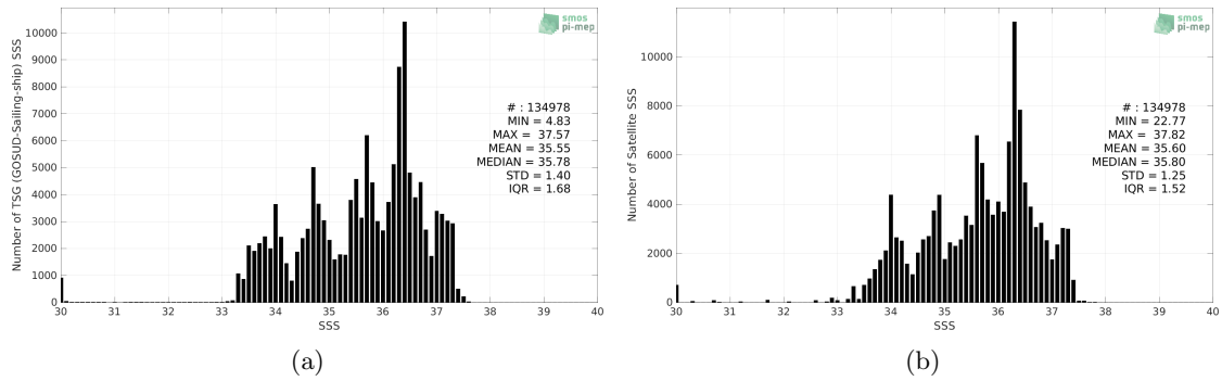
Figure 2: Histograms of SSS from TSG (GOSUD-Sailing-ship) (a) and SMOS SSS L3 v7 - 18 Days (CATDS-CECOS-LOCEAN) (b) considering all match-up pairs per bins of 0.1 over the South Atlantic Ocean Pi-MEP region and for the full satellite product period.
