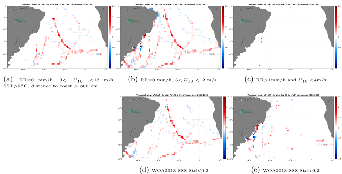
Figure 12: Temporal mean gridded over spatial boxes of size 1^\circ \times 1^\circ of \Delta\text{SSS} (SMOS SSS L3 v7 - 18 Days (CATDS-CECOS-LOCEAN) - TSG (GOSUD-Sailing-ship)) for 5 different subdatasets corresponding to:RR=0 mm/h, 3 < U_{10} < 12 m/s, SST >5^\circ\text{C} , distance to coast > 800 km (a), RR=0 mm/h, 3 < U_{10} < 12 m/s (b), RR >1 mm/h and U_{10} < 4 m/s (c), WOA2013 SSS Std <0.2 (d), WOA2013 SSS Std >0.2 (e).
