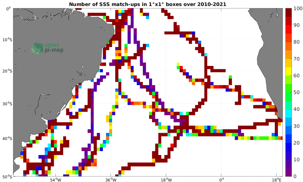
Figure 4: Number of SSS match-ups between TSG (GOSUD-Sailing-ship) SSS and the SMOS SSS L3 v7 - 18 Days (CATDS-CECOS-LOCEAN) SSS product for the South Atlantic Ocean Pi-MEP region over 1^\circ \times 1^\circ boxes and for the full satellite product period.
