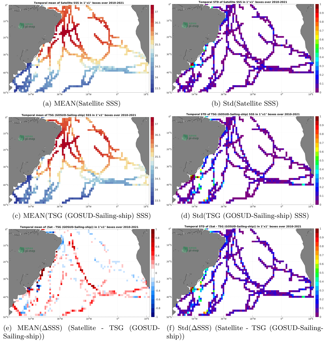
Figure 6: Temporal mean (left) and Std (right) of SSS from SMOS SSS L3 v7 - 18 Days (CATDS-CECOS-LOCEAN) (top), TSG (GOSUD-Sailing-ship) (middle), and of \Delta SSS (Satellite - TSG (GOSUD-Sailing-ship)). Only match-up pairs are used to generate these maps.
