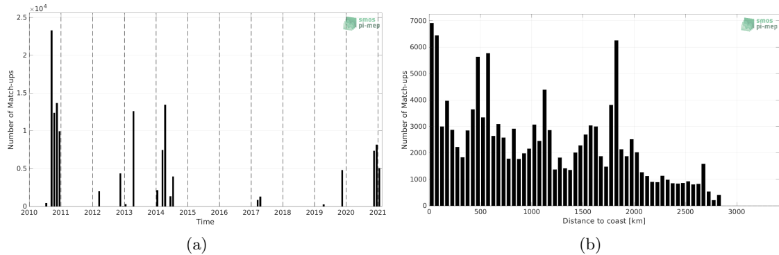
Figure 1: Number of match-ups between TSG (GOSUD-Sailing-ship) and SMOS SSS L3 v7 - 18 Days (CATDS-CECOS-LOCEAN) SSS as a function of time (a) and as function of the distance to coast (b) over the South Atlantic Ocean Pi-MEP region and for the full satellite product period.
