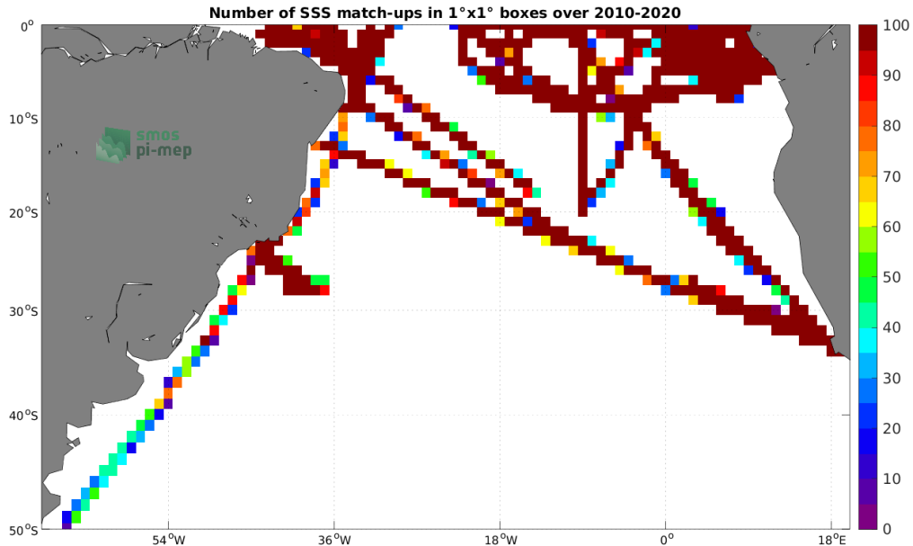
Figure 4: Number of SSS match-ups between TSG (GOSUD-Research-vessel) SSS and the SMOS SSS L3 v7 - 18 Days (CATDS-CECOS-LOCEAN) SSS product for the South Atlantic Ocean Pi-MEP region over 1^\circ \times 1^\circ boxes and for the full satellite product period.
