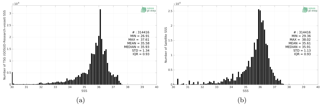
Figure 2: Histograms of SSS from TSG (GOSUD-Research-vessel) (a) and SMOS SSS L3 v7 - 18 Days (CATDS-CECOS-LOCEAN) (b) considering all match-up pairs per bins of 0.1 over the South Atlantic Ocean Pi-MEP region and for the full satellite product period.
