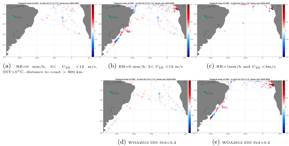
Figure 12: Temporal mean gridded over spatial boxes of size 1^\circ \times 1^\circ of \Delta SSS (SMOS SSS L3 v7 - 18 Days (CATDS-CECOS-LOCEAN) - TSG (GOSUD-Research-vessel)) for 5 different sub-datasets corresponding to:RR=0 mm/h, 3 < U_{10} < 12 m/s, SST>5°C, distance to coast > 800 km (a), RR=0 mm/h, 3 < U_{10} < 12 m/s (b), RR>1mm/h and U_{10} < 4 m/s (c), WOA2013 SSS Std<0.2 (d), WOA2013 SSS Std>0.2 (e).
