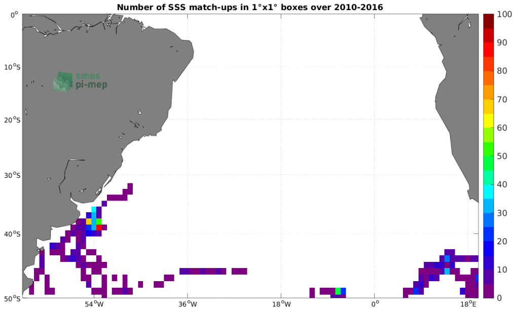
Figure 4: Number of SSS match-ups between Marine mammals SSS and the SMOS SSS L3 v7 - 18 Days (CATDS-CECOS-LOCEAN) SSS product for the South Atlantic Ocean Pi-MEP region over 1^{\circ} \times 1^{\circ} boxes and for the full satellite product period.
