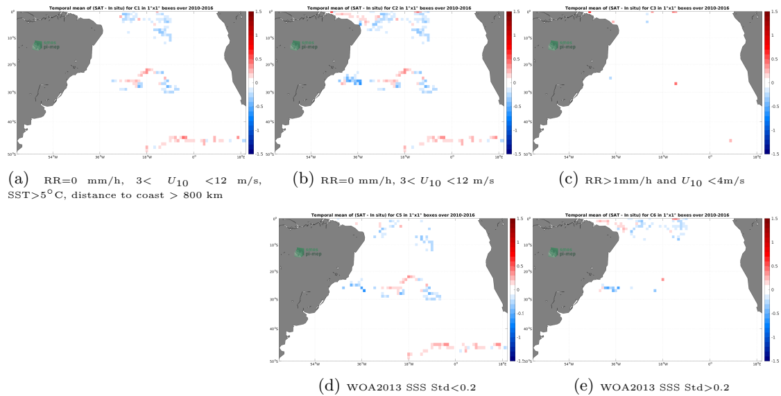
Figure 11: Temporal mean gridded over spatial boxes of size 1^\circ \times 1^\circ of \Delta\text{SSS} (SMOS SSS L3 v7 - 18 Days (CATDS-CECOS-LOCEAN) - Surface drifters) for 5 different subdatasets corresponding to:RR=0 mm/h, 3 < U_{10} < 12 m/s, SST >5^\circ\text{C} , distance to coast > 800 km (a), RR=0 mm/h, 3 < U_{10} < 12 m/s (b), RR >1 mm/h and U_{10} < 4 m/s (c), WOA2013 SSS Std <0.2 (d), WOA2013 SSS Std >0.2 (e).
