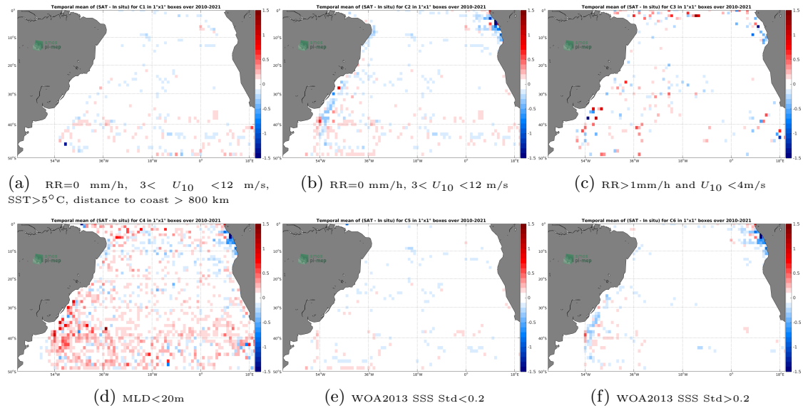
Figure 12: Temporal mean gridded over spatial boxes of size 1^\circ \times 1^\circ of \Delta SSS (SMOS SSS L3 v7 - 18 Days (CATDS-CECOS-LOCEAN) - Argo) for 6 different subdatasets corresponding to:RR=0 mm/h, 3 < U_{10} < 12 m/s, SST >5^\circ C, distance to coast > 800 km (a), RR=0 mm/h, 3 < U_{10} < 12 m/s (b), RR >1 mm/h and U_{10} < 4 m/s (c),MLD <20 m (d),WOA2013 SSS Std <0.2 (e),WOA2013 SSS Std >0.2 (f).
