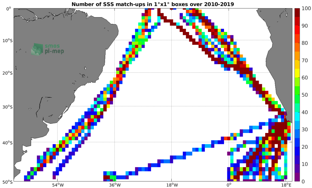
Figure 4: Number of SSS match-ups between TSG (Polarstern) SSS and the SMOS SSS L3 v5 - 9 Days (CATDS-CECOS-LOCEAN) SSS product for the South Atlantic Ocean Pi-MEP region over 1^{\circ} \times 1^{\circ} boxes and for the full satellite product period.
