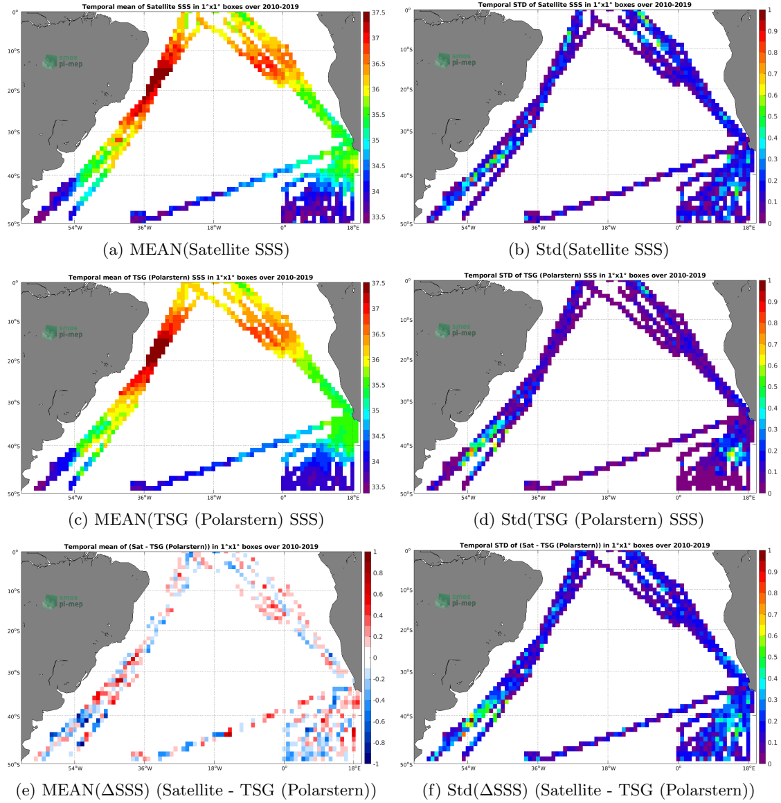
Figure 6: Temporal mean (left) and Std (right) of SSS from SMOS SSS L3 v5 - 9 Days (CATDS-CECOS-LOCEAN) (top), TSG (Polarstern) (middle), and of \Delta SSS (Satellite - TSG (Polarstern)). Only match-up pairs are used to generate these maps.
