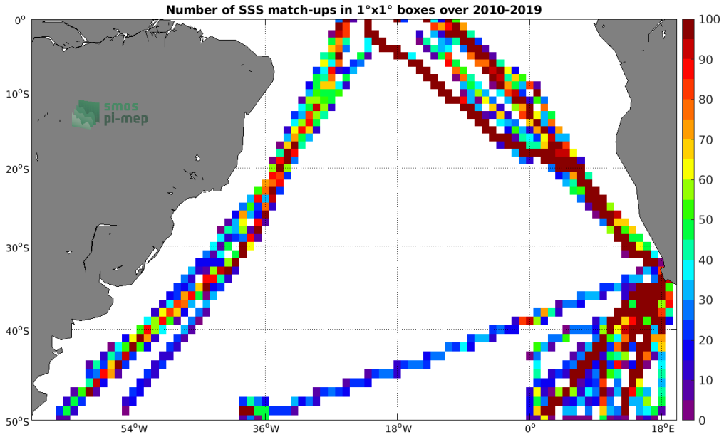
Figure 4: Number of SSS match-ups between TSG (Polarstern) SSS and the SMOS SSS L3 v5 - 9 Days (CATDS-CECOS-LOCEAN) SSS product for the South Atlantic Ocean Pi-MEP region over 1°x1° boxes and for the full satellite product period.
