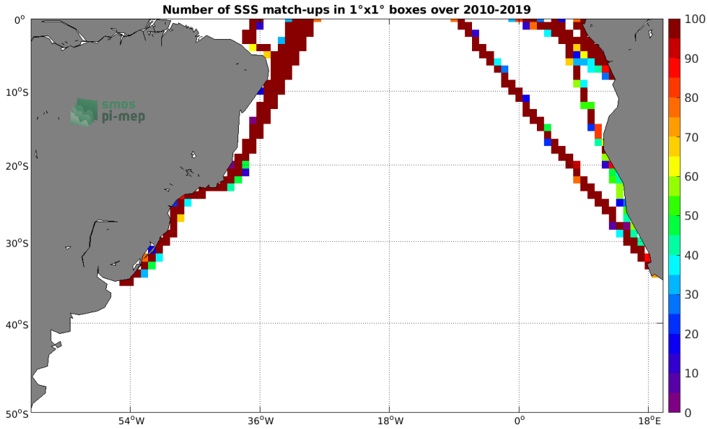
Figure 4: Number of SSS match-ups between TSG (LEGOS-DM) SSS and the SMOS SSS L3 v5 - 9 Days (CATDS-CECOS-LOCEAN) SSS product for the South Atlantic Ocean Pi-MEP region over 1°x1° boxes and for the full satellite product period.
