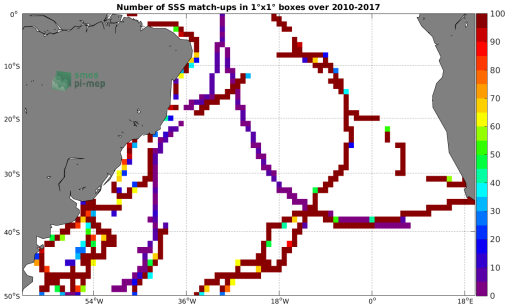
Figure 4: Number of SSS match-ups between TSG (GOSUD-Sailing-ship) SSS and the SMOS SSS L3 v5 - 9 Days (CATDS-CECOS-LOCEAN) SSS product for the South Atlantic Ocean Pi-MEP region over 1^\circ \times 1^\circ boxes and for the full satellite product period.
