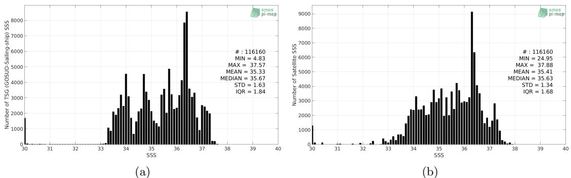
Figure 2: Histograms of SSS from TSG (GOSUD-Sailing-ship) (a) and SMOS SSS L3 v5 - 9 Days (CATDS-CECOS-LOCEAN) (b) considering all match-up pairs per bins of 0.1 over the South Atlantic Ocean Pi-MEP region and for the full satellite product period.
