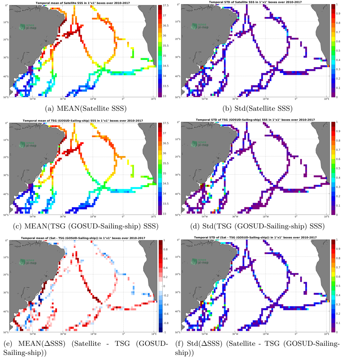
Figure 6: Temporal mean (left) and Std (right) of SSS from SMOS SSS L3 v5 - 9 Days (CATDS-CECOS-LOCEAN) (top), TSG (GOSUD-Sailing-ship) (middle), and of \Delta SSS (Satellite - TSG (GOSUD-Sailing-ship)). Only match-up pairs are used to generate these maps.
