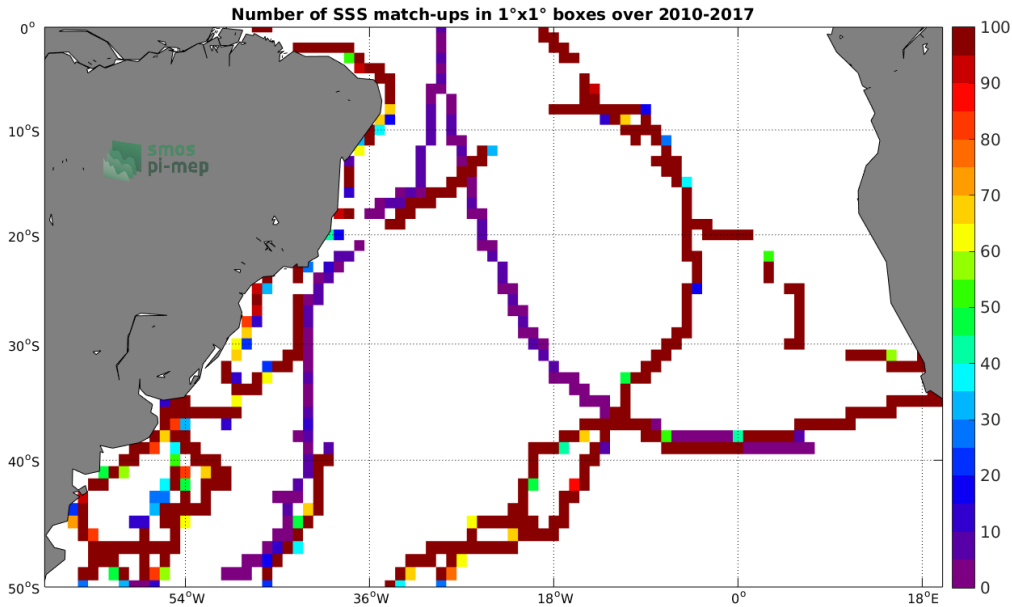
Figure 4: Number of SSS match-ups between TSG (GOSUD-Sailing-ship) SSS and the SMOS SSS L3 v5 - 9 Days (CATDS-CECOS-LOCEAN) SSS product for the South Atlantic Ocean Pi-MEP region over 1^{\circ} \times 1^{\circ} boxes and for the full satellite product period.
