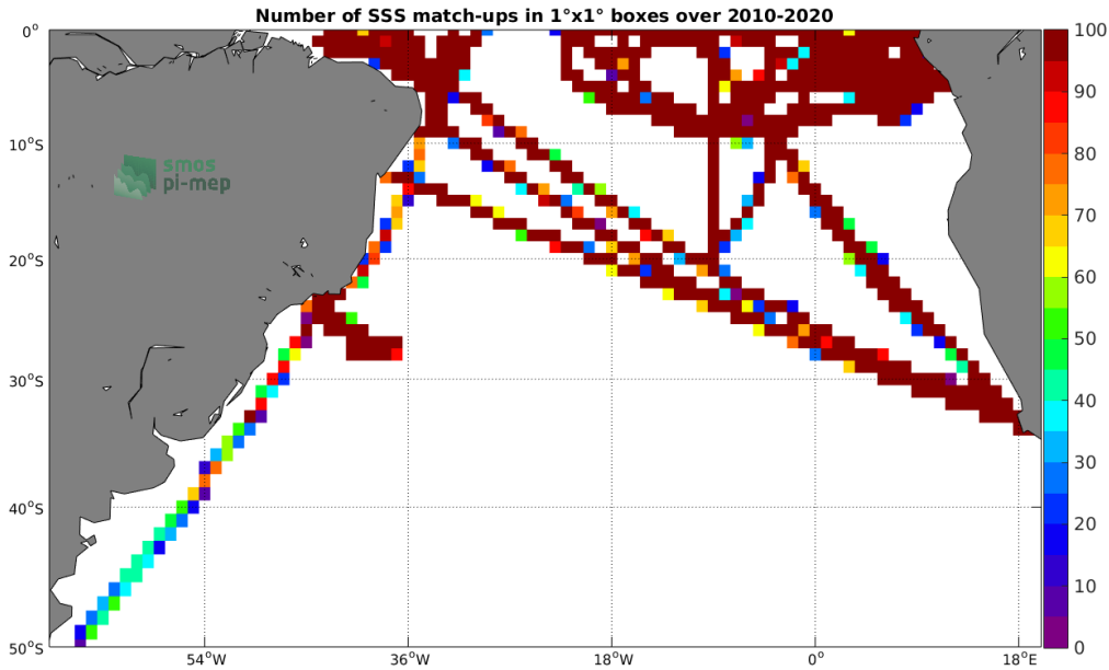
Figure 4: Number of SSS match-ups between TSG (GOSUD-Research-vessel) SSS and the SMOS SSS L3 v5 - 9 Days (CATDS-CECOS-LOCEAN) SSS product for the South Atlantic Ocean Pi-MEP region over 1^{\circ} \times 1^{\circ} boxes and for the full satellite product period.
