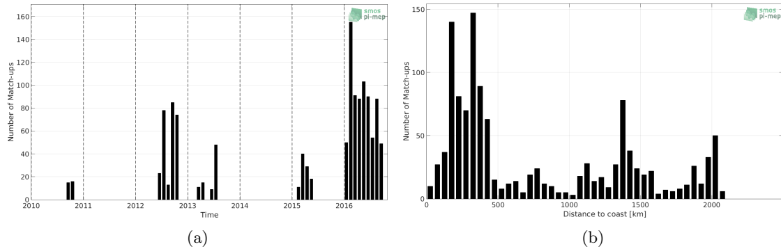
Figure 1: Number of match-ups between Marine mammals and SMOS SSS L3 v5 - 9 Days (CATDS-CECOS-LOCEAN) SSS as a function of time (a) and as function of the distance to coast (b) over the South Atlantic Ocean Pi-MEP region and for the full satellite product period.
