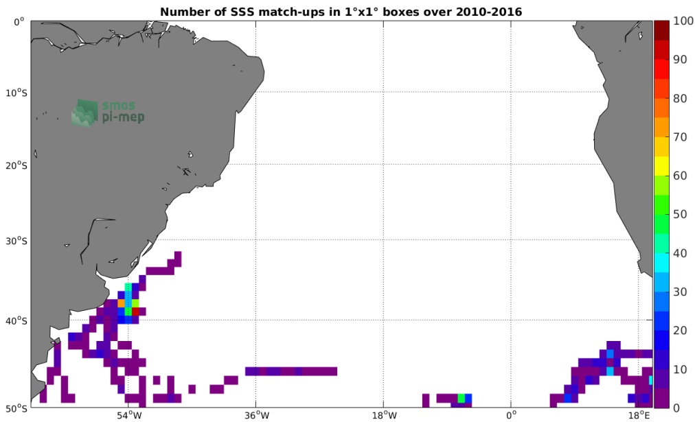
Figure 4: Number of SSS match-ups between Marine mammals SSS and the SMOS SSS L3 v5 - 9 Days (CATDS-CECOS-LOCEAN) SSS product for the South Atlantic Ocean Pi-MEP region over 1^\circ \times 1^\circ boxes and for the full satellite product period.
