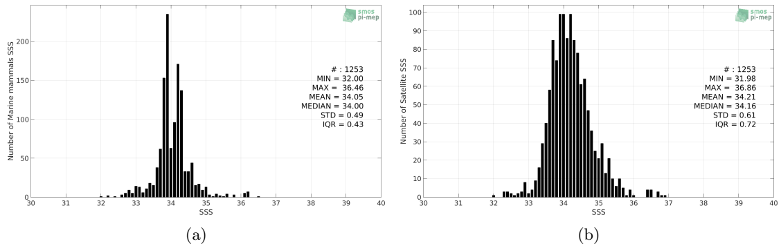
Figure 2: Histograms of SSS from Marine mammals (a) and SMOS SSS L3 v5 - 9 Days (CATDS-CECOS-LOCEAN) (b) considering all match-up pairs per bins of 0.1 over the South Atlantic Ocean Pi-MEP region and for the full satellite product period.
