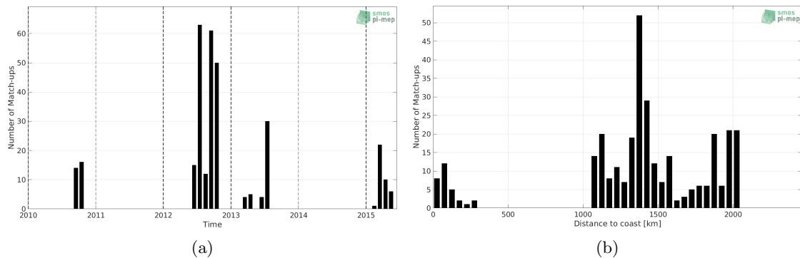
Figure 1: Number of match-ups between Sea mammals and SMOS SSS L3 v5 - 9 Days (CATDS-CECOS-LOCEAN) SSS as a function of time (a) and as function of the distance to coast (b) over the South Atlantic Ocean Pi-MEP region and for the full satellite product period.
