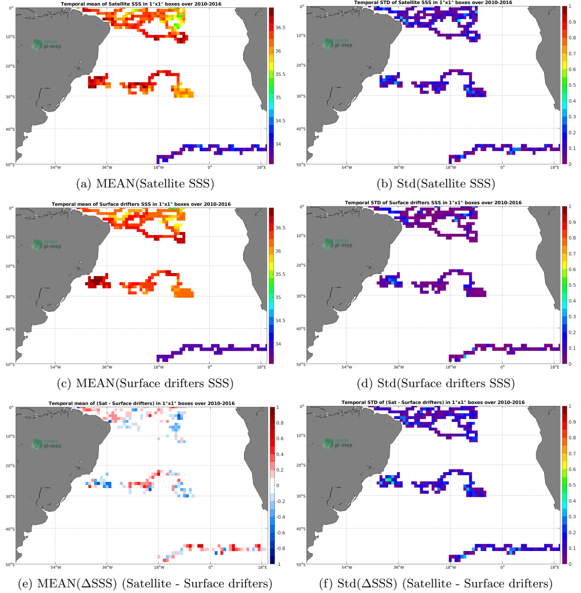
Figure 5: Temporal mean (left) and Std (right) of SSS from SMOS SSS L3 v5 - 9 Days (CATDS-CECOS-LOCEAN) (top), Surface drifters (middle), and of \Delta SSS (Satellite - Surface drifters). Only match-up pairs are used to generate these maps.
