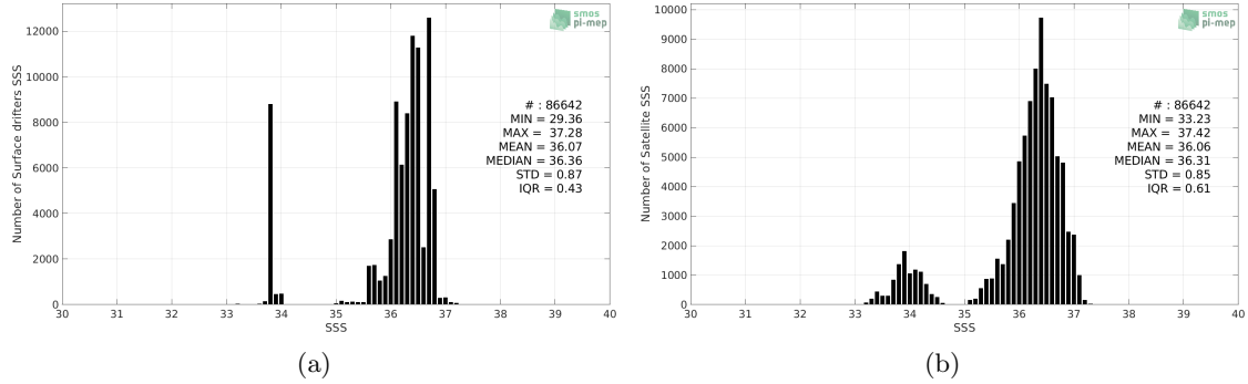
Figure 2: Histograms of SSS from Surface drifters (a) and SMOS SSS L3 v5 - 9 Days (CATDS-CECOS-LOCEAN) (b) considering all match-up pairs per bins of 0.1 over the South Atlantic Ocean Pi-MEP region and for the full satellite product period.
