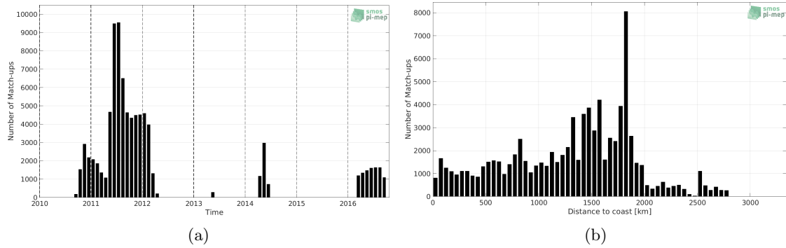
Figure 1: Number of match-ups between Surface drifters and SMOS SSS L3 v5 - 9 Days (CATDS-CECOS-LOCEAN) SSS as a function of time (a) and as function of the distance to coast (b) over the South Atlantic Ocean Pi-MEP region and for the full satellite product period.
