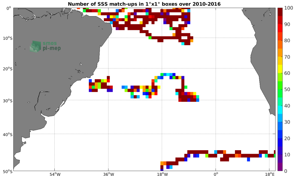
Figure 3: Number of SSS match-ups between Surface drifters SSS and the SMOS SSS L3 v5 - 9 Days (CATDS-CECOS-LOCEAN) SSS product for the South Atlantic Ocean Pi-MEP region over 1^\circ \times 1^\circ boxes and for the full satellite product period.
