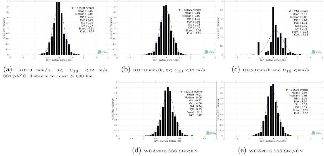
Figure 12: Normalized histogram of \Delta SSS (SMOS SSS L3 v5 - 9 Days (CATDS-CECOS-LOCEAN) - Surface drifters) for 5 different subdatasets corresponding to: RR=0 mm/h, 3 < U_{10} < 12 m/s, SST>5°C, distance to coast > 800 km (a), RR=0 mm/h, 3 < U_{10} < 12 m/s (b), RR>1mm/h and U_{10} < 4 m/s (c), WOA2013 SSS Std<0.2 (d), WOA2013 SSS Std>0.2 (e).
