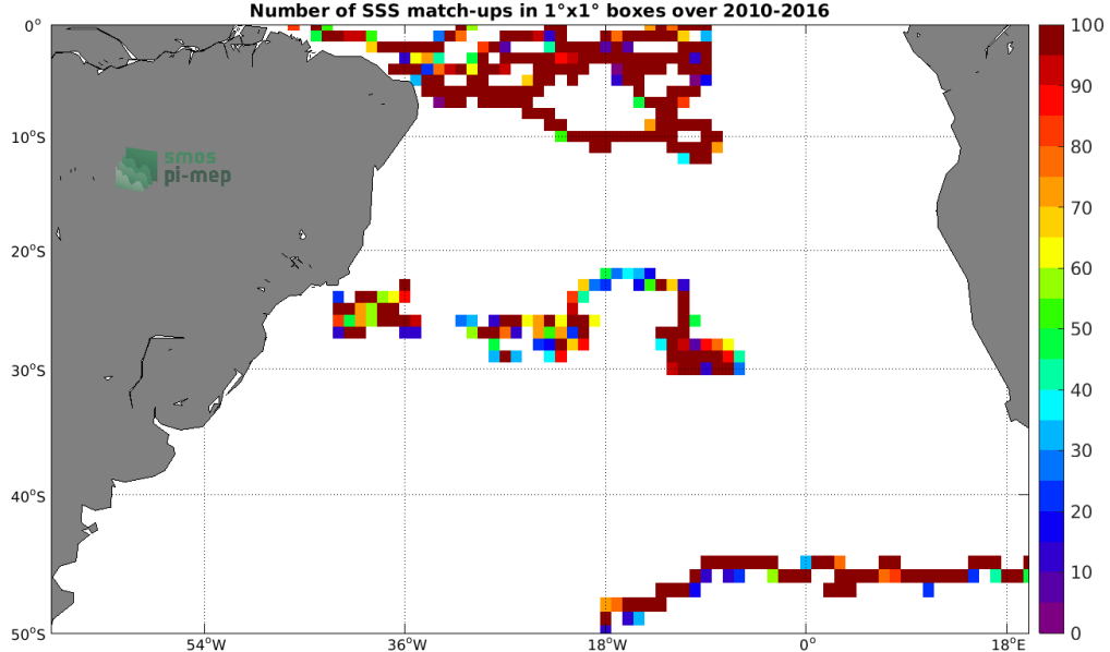
Figure 3: Number of SSS match-ups between Surface drifters SSS and the SMOS SSS L3 v5 - 9 Days (CATDS-CECOS-LOCEAN) SSS product for the South Atlantic Ocean Pi-MEP region over 1^\circ \times 1^\circ boxes and for the full satellite product period.
