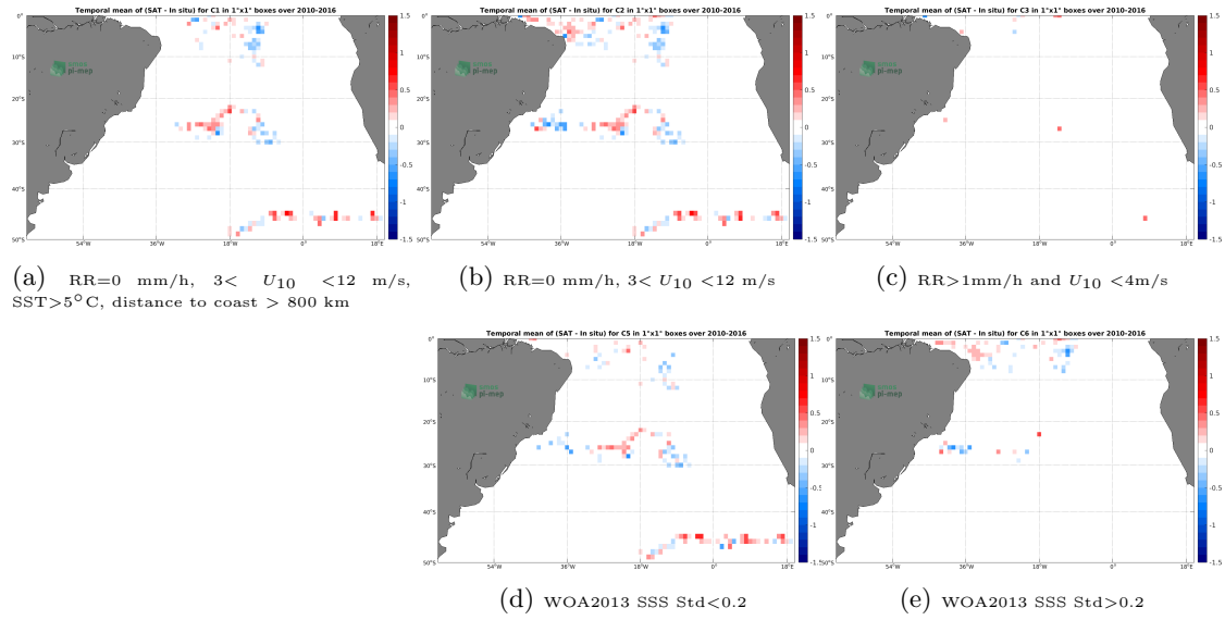
Figure 11: Temporal mean gridded over spatial boxes of size 1^\circ \times 1^\circ of \Delta SSS (SMOS SSS L3 v5 - 9 Days (CATDS-CECOS-LOCEAN) - Surface drifters) for 5 different subdatasets corresponding to: RR=0 mm/h, 3 < U_{10} < 12 m/s, SST > 5^\circ C , distance to coast > 800 km (a), RR=0 mm/h, 3 < U_{10} < 12 m/s (b), RR > 1 mm/h and U_{10} < 4 m/s (c), WOA2013 SSS Std < 0.2 (d), WOA2013 SSS Std > 0.2 (e).
