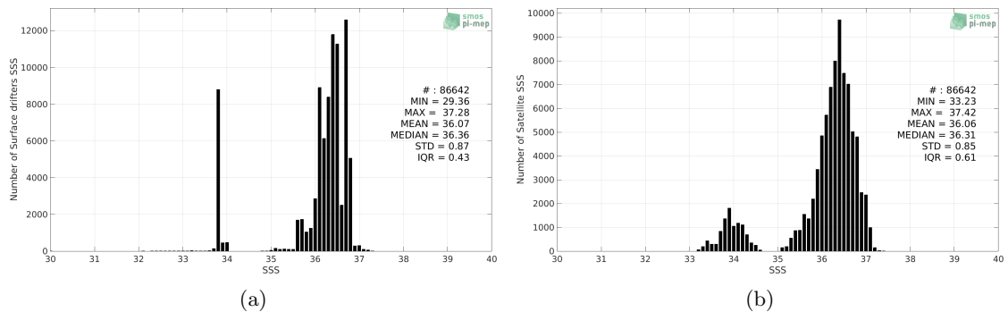
Figure 2: Histograms of SSS from Surface drifters (a) and SMOS SSS L3 v5 - 9 Days (CATDS-CECOS-LOCEAN) (b) considering all match-up pairs per bins of 0.1 over the South Atlantic Ocean Pi-MEP region and for the full satellite product period.
