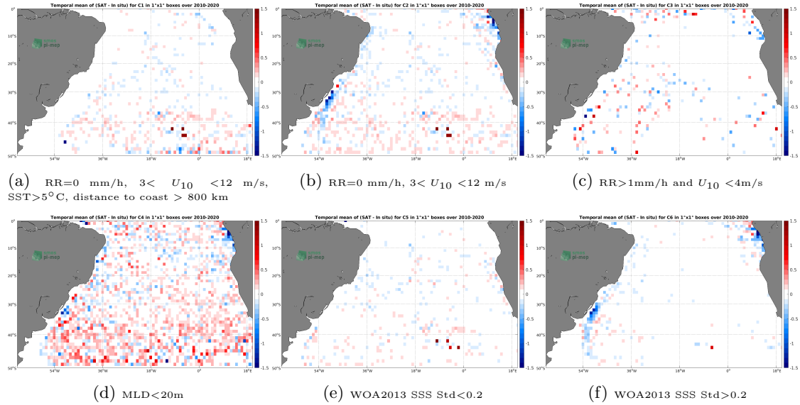
Figure 12: Temporal mean gridded over spatial boxes of size 1^\circ \times 1^\circ of \Delta SSS (SMOS SSS L3 v5 - 9 Days (CATDS-CECOS-LOCEAN) - Argo) for 6 different subdatasets corresponding to: RR=0 mm/h, 3 < U_{10} < 12 m/s, SST > 5^\circ C , distance to coast > 800 km (a), RR=0 mm/h, 3 < U_{10} < 12 m/s (b), RR > 1 mm/h and U_{10} < 4 m/s (c), MLD < 20 m (d), WOA2013 SSS Std < 0.2 (e), WOA2013 SSS Std > 0.2 (f).
