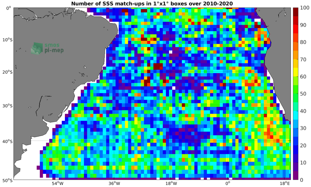
Figure 4: Number of SSS match-ups between Argo SSS and the SMOS SSS L3 v5 - 9 Days (CATDS-CECOS-LOCEAN) SSS product for the South Atlantic Ocean Pi-MEP region over 1^\circ \times 1^\circ boxes and for the full satellite product period.
