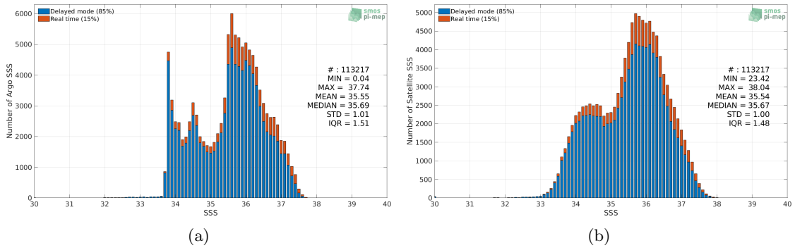
Figure 2: Histograms of SSS from Argo (a) and SMOS SSS L3 v5 - 9 Days (CATDS-CECOS-LOCEAN) (b) considering all match-up pairs per bins of 0.1 over the South Atlantic Ocean Pi-MEP region and for the full satellite product period.
