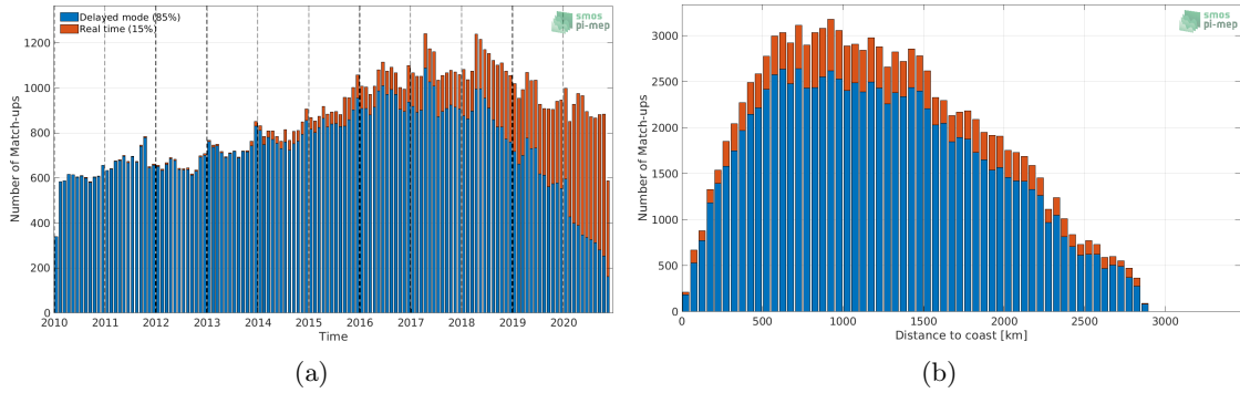
Figure 1: Number of match-ups between Argo and SMOS SSS L3 v5 - 9 Days (CATDS-CECOS-LOCEAN) SSS as a function of time (a) and as function of the distance to coast (b) over the South Atlantic Ocean Pi-MEP region and for the full satellite product period.
