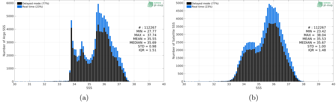
Figure 2: Histograms of SSS from Argo (a) and SMOS SSS L3 v5 - 9 Days (CATDS-CECOS-LOCEAN) (b) considering all match-up pairs per bins of 0.1 over the South Atlantic Ocean Pi-MEP region and for the full satellite product period.
