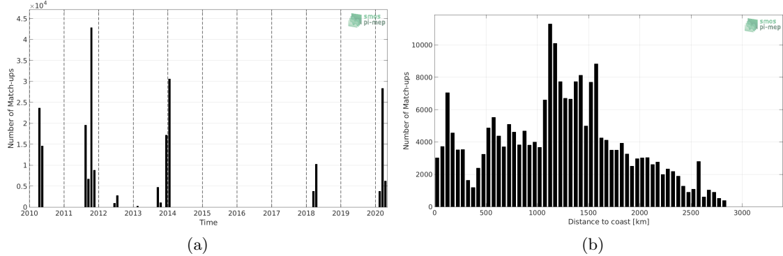
Figure 1: Number of match-ups between TSG (SAMOS) and SMOS SSS L3 v5 - 18 Days (CATDS-CECOS-LOCEAN) SSS as a function of time (a) and as function of the distance to coast (b) over the South Atlantic Ocean Pi-MEP region and for the full satellite product period.
