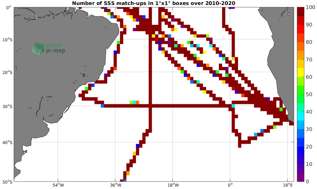
Figure 4: Number of SSS match-ups between TSG (SAMOS) SSS and the SMOS SSS L3 v5 - 18 Days (CATDS-CECOS-LOCEAN) SSS product for the South Atlantic Ocean Pi-MEP region over 1^\circ \times 1^\circ boxes and for the full satellite product period.
