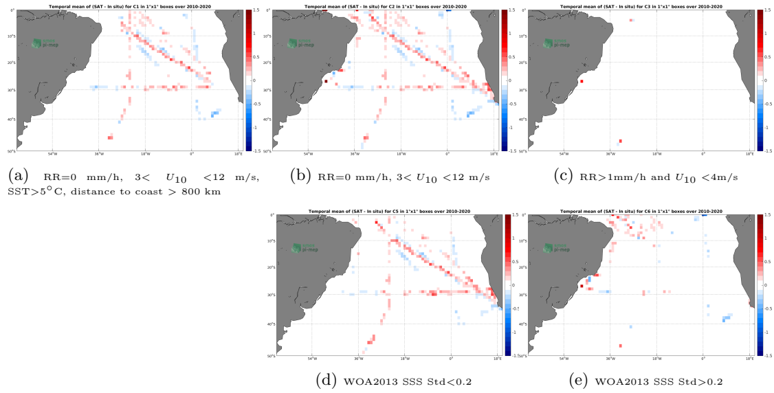
Figure 12: Temporal mean gridded over spatial boxes of size 1^\circ \times 1^\circ of \Delta SSS (SMOS SSS L3 v5 - 18 Days (CATDS-CECOS-LOCEAN) - TSG (SAMOS)) for 5 different subdatasets corresponding to:RR=0 mm/h, 3 < U_{10} < 12 m/s, SST >5^\circ\text{C} , distance to coast > 800 km (a), RR=0 mm/h, 3 < U_{10} < 12 m/s (b), RR >1 mm/h and U_{10} < 4 m/s (c), WOA2013 SSS Std <0.2 (d), WOA2013 SSS Std >0.2 (e).
