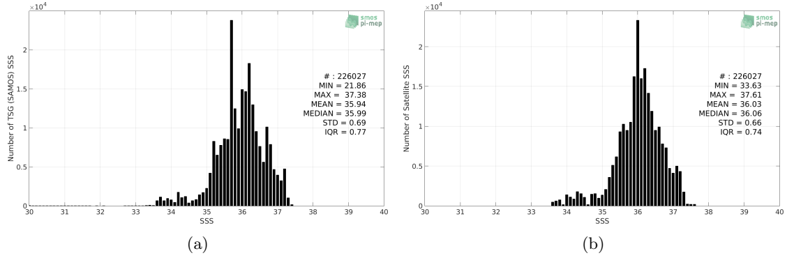
Figure 2: Histograms of SSS from TSG (SAMOS) (a) and SMOS SSS L3 v5 - 18 Days (CATDS-CECOS-LOCEAN) (b) considering all match-up pairs per bins of 0.1 over the South Atlantic Ocean Pi-MEP region and for the full satellite product period.
