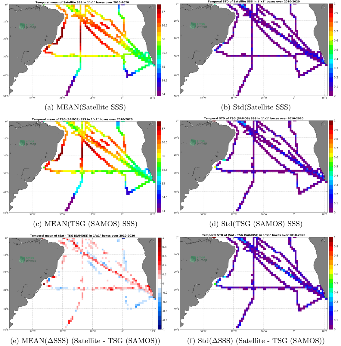
Figure 6: Temporal mean (left) and Std (right) of SSS from SMOS SSS L3 v5 - 18 Days (CATDS-CECOS-LOCEAN) (top), TSG (SAMOS) (middle), and of \Delta SSS (Satellite - TSG (SAMOS)). Only match-up pairs are used to generate these maps.
