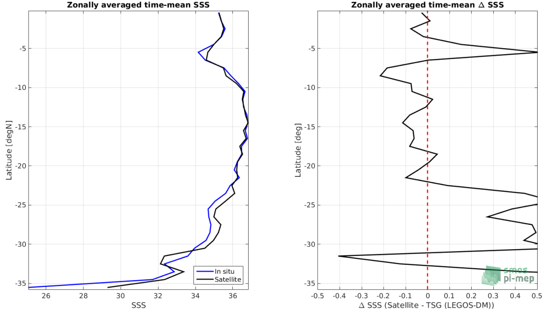
Figure 8: Left panel: Zonal mean SSS from SMOS SSS L3 v5 - 18 Days (CATDS-CECOS-LOCEAN) satellite product (black) and from TSG (LEGOS-DM) (blue). Right panel: Zonal mean of \Delta\text{SSS} (Satellite - TSG (LEGOS-DM)) for all the collected Pi-MEP match-up pairs estimated over the full satellite product period.
