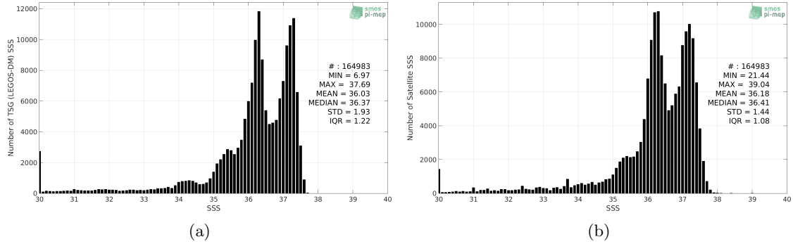
Figure 2: Histograms of SSS from TSG (LEGOS-DM) (a) and SMOS SSS L3 v5 - 18 Days (CATDS-CECOS-LOCEAN) (b) considering all match-up pairs per bins of 0.1 over the South Atlantic Ocean Pi-MEP region and for the full satellite product period.
