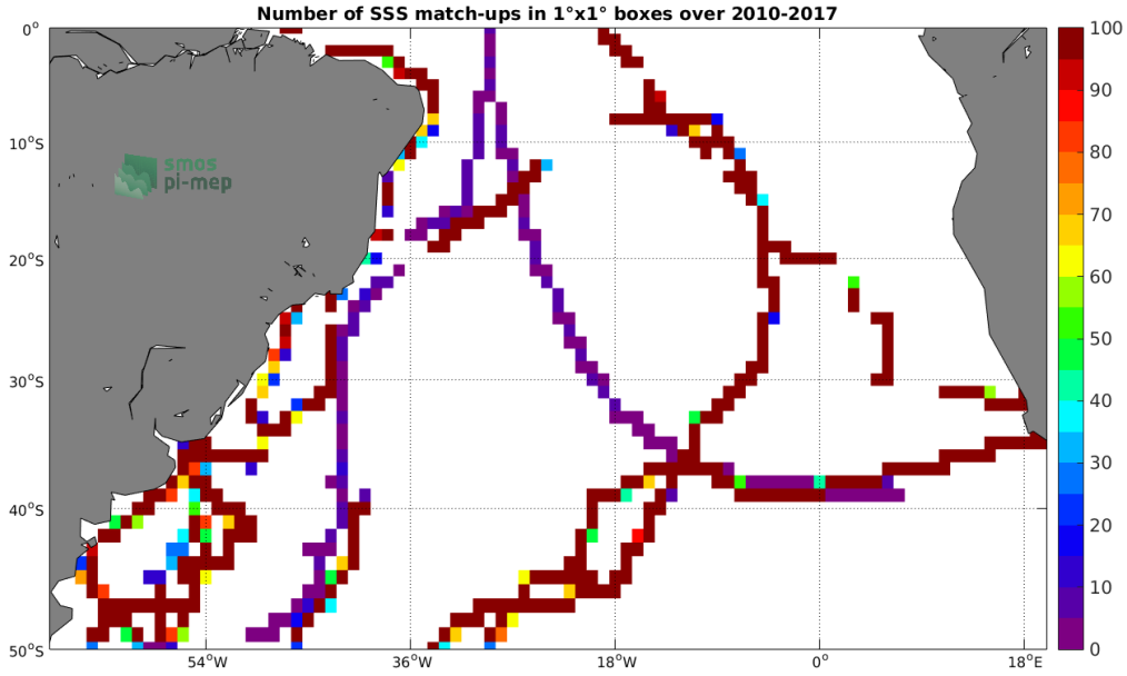
Figure 4: Number of SSS match-ups between TSG (GOSUD-Sailing-ship) SSS and the SMOS SSS L3 v5 - 18 Days (CATDS-CECOS-LOCEAN) SSS product for the South Atlantic Ocean Pi-MEP region over 1^\circ \times 1^\circ boxes and for the full satellite product period.
