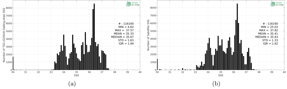
Figure 2: Histograms of SSS from TSG (GOSUD-Sailing-ship) (a) and SMOS SSS L3 v5 - 18 Days (CATDS-CECOS-LOCEAN) (b) considering all match-up pairs per bins of 0.1 over the South Atlantic Ocean Pi-MEP region and for the full satellite product period.
