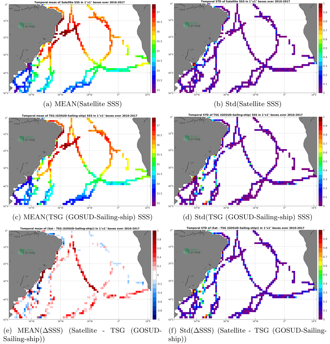
Figure 6: Temporal mean (left) and Std (right) of SSS from SMOS SSS L3 v5 - 18 Days (CATDS-CECOS-LOCEAN) (top), TSG (GOSUD-Sailing-ship) (middle), and of \Delta SSS (Satellite - TSG (GOSUD-Sailing-ship)). Only match-up pairs are used to generate these maps.
