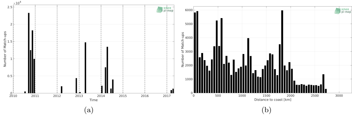
Figure 1: Number of match-ups between TSG (GOSUD-Sailing-ship) and SMOS SSS L3 v5 - 18 Days (CATDS-CECOS-LOCEAN) SSS as a function of time (a) and as function of the distance to coast (b) over the South Atlantic Ocean Pi-MEP region and for the full satellite product period.
