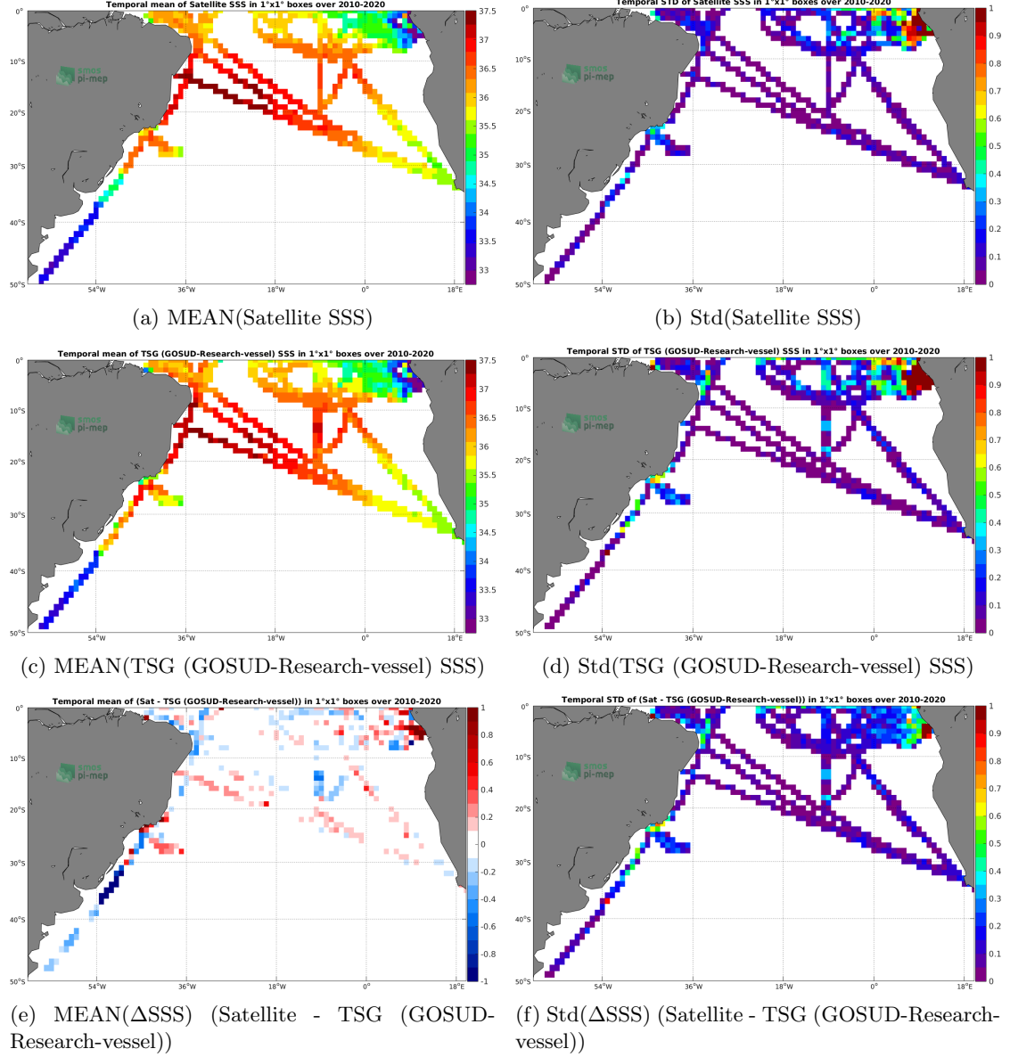
Figure 6: Temporal mean (left) and Std (right) of SSS from SMOS SSS L3 v5 - 18 Days (CATDS-CECOS-LOCEAN) (top), TSG (GOSUD-Research-vessel) (middle), and of \Delta SSS (Satellite - TSG (GOSUD-Research-vessel)). Only match-up pairs are used to generate these maps.
