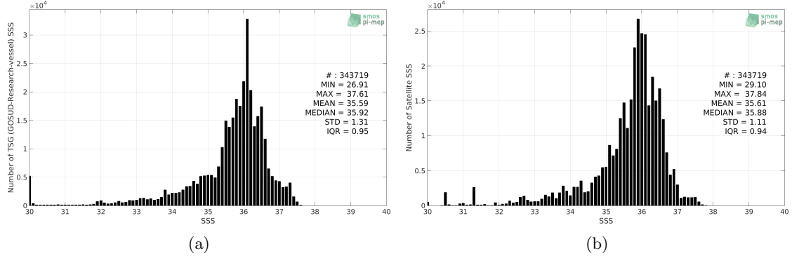
Figure 2: Histograms of SSS from TSG (GOSUD-Research-vessel) (a) and SMOS SSS L3 v5 - 18 Days (CATDS-CECOS-LOCEAN) (b) considering all match-up pairs per bins of 0.1 over the South Atlantic Ocean Pi-MEP region and for the full satellite product period.
