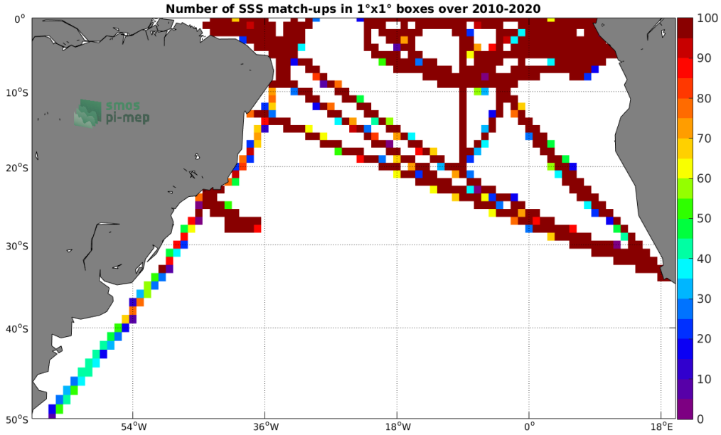
Figure 4: Number of SSS match-ups between TSG (GOSUD-Research-vessel) SSS and the SMOS SSS L3 v5 - 18 Days (CATDS-CECOS-LOCEAN) SSS product for the South Atlantic Ocean Pi-MEP region over 1^\circ \times 1^\circ boxes and for the full satellite product period.
