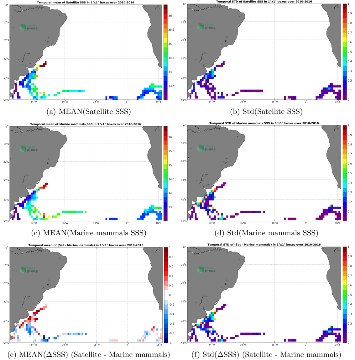
Figure 6: Temporal mean (left) and Std (right) of SSS from SMOS SSS L3 v5 - 18 Days (CATDS-CECOS-LOCEAN) (top), Marine mammals (middle), and of \Delta SSS (Satellite - Marine mammals). Only match-up pairs are used to generate these maps.
