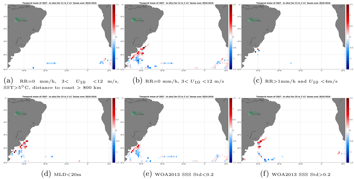
Figure 12: Temporal mean gridded over spatial boxes of size 1^{\circ} \times 1^{\circ} of \Delta\text{SSS} (SMOS SSS L3 v5 - 18 Days (CATDS-CECOS-LOCEAN) - Marine mammals) for 6 different subdatasets corresponding to: RR=0 mm/h, 3 < U_{10} < 12 m/s, SST >5^{\circ}\text{C} , distance to coast > 800 km (a), RR=0 mm/h, 3 < U_{10} < 12 m/s (b), RR >1\text{mm/h} and U_{10} < 4\text{m/s} (c), MLD <20\text{m} (d), WOA2013 SSS Std <0.2 (e), WOA2013 SSS Std >0.2 (f).
