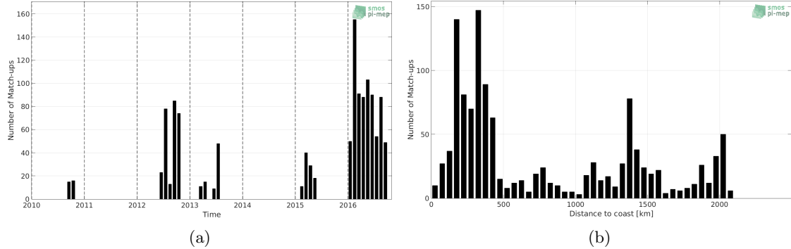
Figure 1: Number of match-ups between Marine mammals and SMOS SSS L3 v5 - 18 Days (CATDS-CECOS-LOCEAN) SSS as a function of time (a) and as function of the distance to coast (b) over the South Atlantic Ocean Pi-MEP region and for the full satellite product period.
