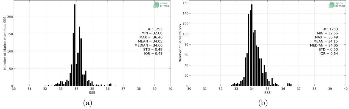
Figure 2: Histograms of SSS from Marine mammals (a) and SMOS SSS L3 v5 - 18 Days (CATDS-CECOS-LOCEAN) (b) considering all match-up pairs per bins of 0.1 over the South Atlantic Ocean Pi-MEP region and for the full satellite product period.
