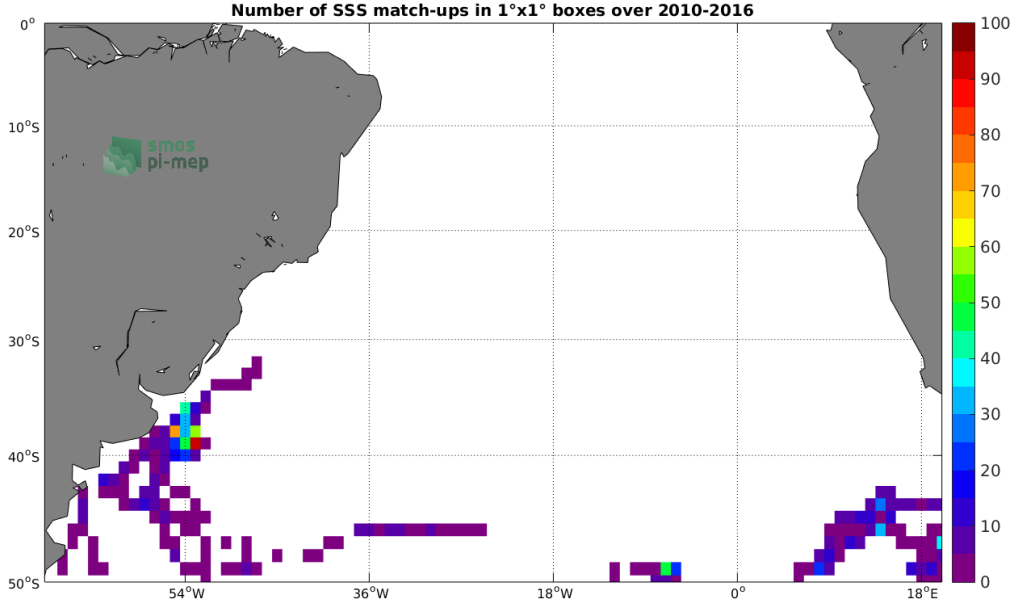
Figure 4: Number of SSS match-ups between Marine mammals SSS and the SMOS SSS L3 v5 - 18 Days (CATDS-CECOS-LOCEAN) SSS product for the South Atlantic Ocean Pi-MEP region over 1^\circ \times 1^\circ boxes and for the full satellite product period.
