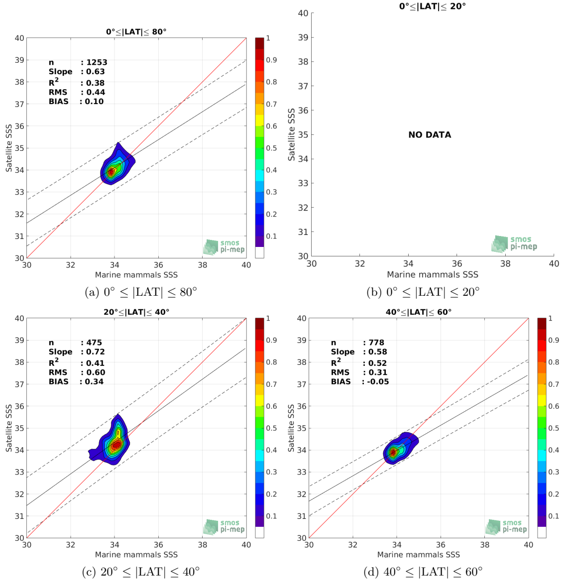
Figure 9: Contour maps of the concentration of SMOS SSS L3 v5 - 18 Days (CATDS-CECOS-LOCEAN) SSS (y-axis) versus Marine mammals SSS (x-axis) at match-up pairs for different latitude bands. For each plot, the red line shows x=y . The black thin and dashed lines indicate a linear fit through the data cloud and the \pm 95\% confidence levels, respectively. The number match-up pairs n , the slope and R^2 coefficient of the linear fit, the root mean square (RMS) and the mean bias between satellite and in situ data are indicated for each latitude band in each plots.
