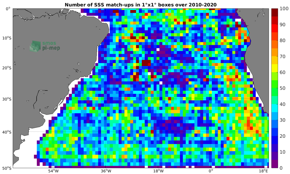
Figure 4: Number of SSS match-ups between Argo SSS and the SMOS SSS L3 v5 - 18 Days (CATDS-CECOS-LOCEAN) SSS product for the South Atlantic Ocean Pi-MEP region over 1°x1° boxes and for the full satellite product period.
