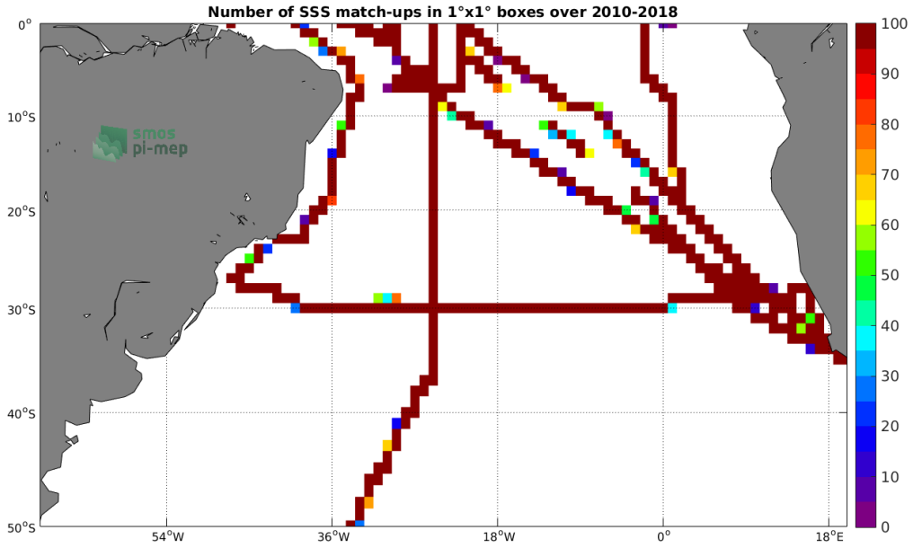
Figure 4: Number of SSS match-ups between TSG (SAMOS) SSS and the SMOS SSS L3 v4 - 9 Days (CATDS-CECOS-LOCEAN) SSS product for the South Atlantic Ocean Pi-MEP region over 1^\circ \times 1^\circ boxes and for the full satellite product period.
