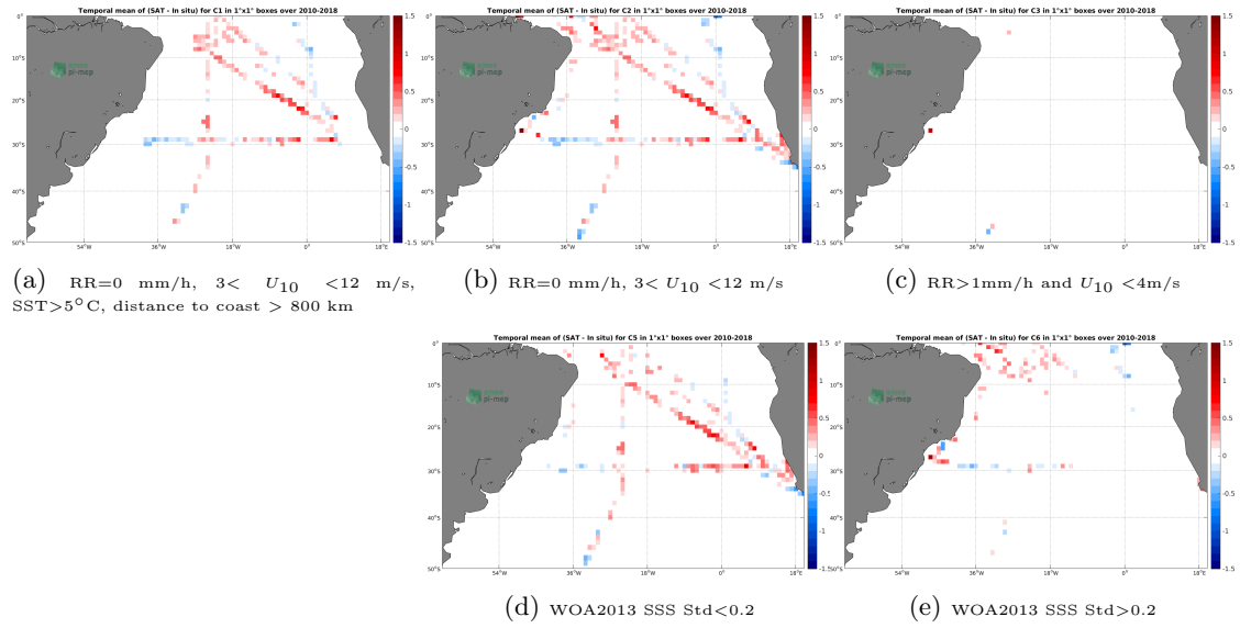
Figure 12: Temporal mean gridded over spatial boxes of size 1^\circ \times 1^\circ of \Delta SSS (SMOS SSS L3 v4 - 9 Days (CATDS-CECOS-LOCEAN) - TSG (SAMOS)) for 5 different subdatasets corresponding to: RR=0 mm/h, 3 < U_{10} < 12 m/s, SST > 5^\circ C , distance to coast > 800 km (a), RR=0 mm/h, 3 < U_{10} < 12 m/s (b), RR > 1 mm/h and U_{10} < 4 m/s (c), WOA2013 SSS Std < 0.2 (d), WOA2013 SSS Std > 0.2 (e).
