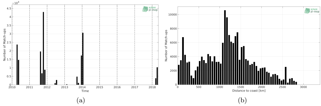
Figure 1: Number of match-ups between TSG (SAMOS) and SMOS SSS L3 v4 - 9 Days (CATDS-CECOS-LOCEAN) SSS as a function of time (a) and as function of the distance to coast (b) over the South Atlantic Ocean Pi-MEP region and for the full satellite product period.
