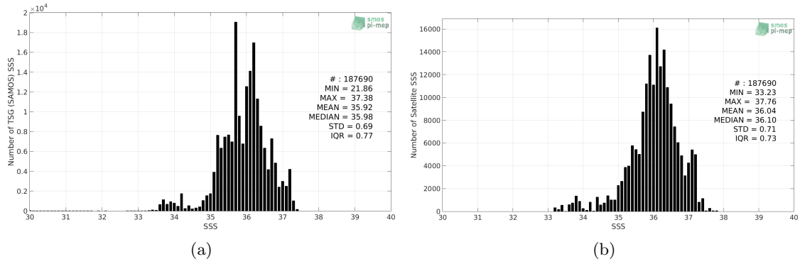
Figure 2: Histograms of SSS from TSG (SAMOS) (a) and SMOS SSS L3 v4 - 9 Days (CATDS-CECOS-LOCEAN) (b) considering all match-up pairs per bins of 0.1 over the South Atlantic Ocean Pi-MEP region and for the full satellite product period.
