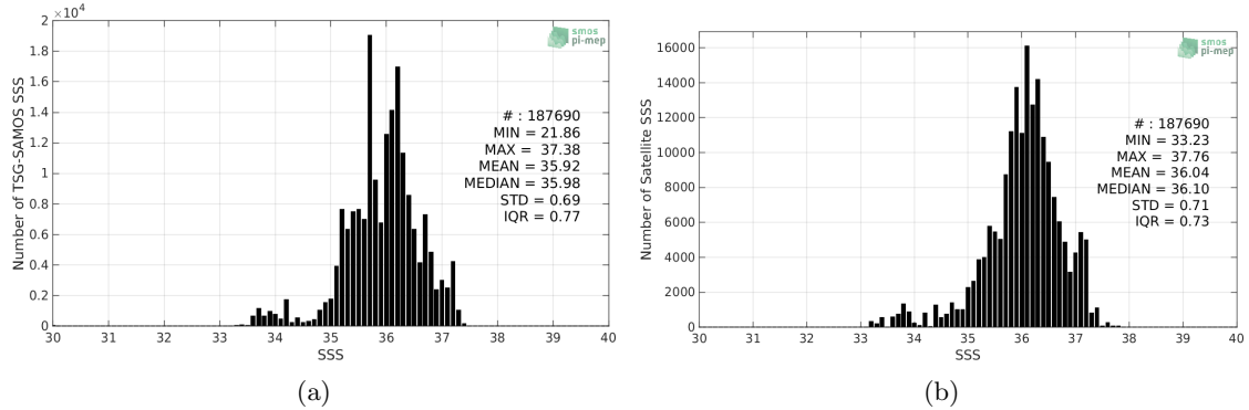
Figure 2: Histograms of SSS from TSG-SAMOS (a) and SMOS-L3-CATDS-CECOS-LOCEAN-V4-9DAYS-25KM (b) considering all match-up pairs per bins of 0.1 over the South Atlantic Ocean Pi-MEP region and for the full satellite product period.
