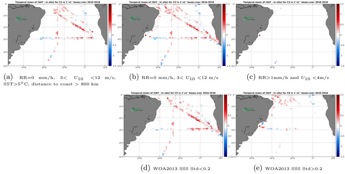
Figure 12: Temporal mean gridded over spatial boxes of size 1^\circ \times 1^\circ of \Delta SSS (SMOS-L3-CATDS-CECOS-LOCEAN-V4-9DAYS-25KM - TSG-SAMOS) for 5 different subdatasets corresponding to: RR=0 mm/h, 3 < U_{10} < 12 m/s, SST > 5^\circ C , distance to coast > 800 km (a), RR=0 mm/h, 3 < U_{10} < 12 m/s (b), RR > 1 mm/h and U_{10} < 4 m/s (c), WOA2013 SSS Std < 0.2 (d), WOA2013 SSS Std > 0.2 (e).
