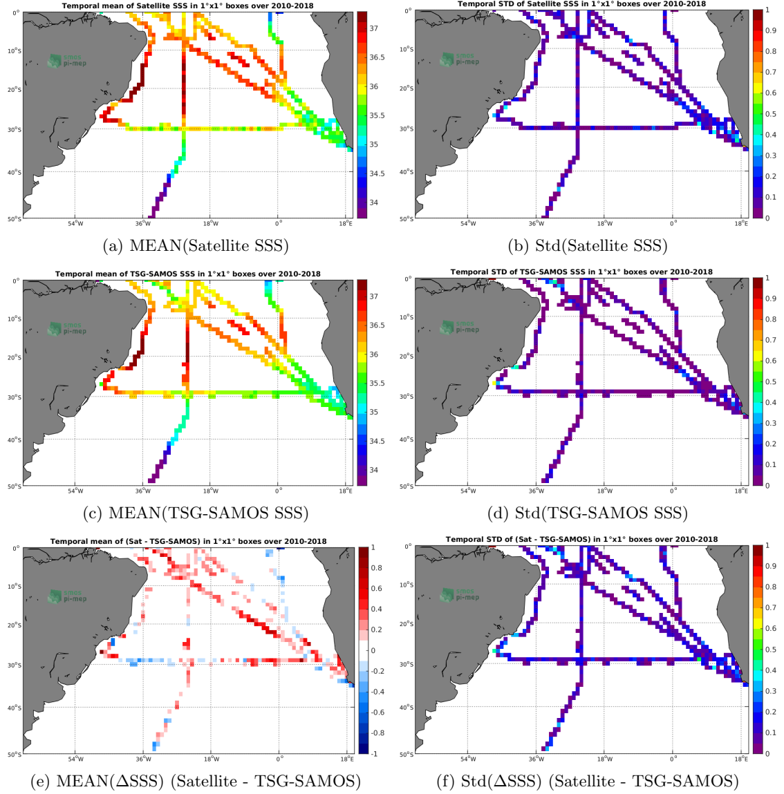
Figure 6: Temporal mean (left) and Std (right) of SSS from SMOS-L3-CATDS-CECOS-LOCEAN-V4-9DAYS-25KM (top), TSG-SAMOS (middle), and of \Delta SSS (Satellite - TSG-SAMOS). Only match-up pairs are used to generate these maps.
