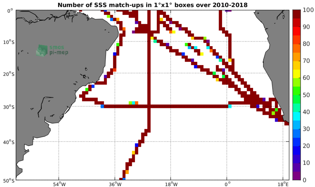
Figure 4: Number of SSS match-ups between TSG-SAMOS SSS and the SMOS-L3-CATDS-CECOS-LOCEAN-V4-9DAYS-25KM SSS product for the South Atlantic Ocean Pi-MEP region over 1^\circ \times 1^\circ boxes and for the full satellite product period.
