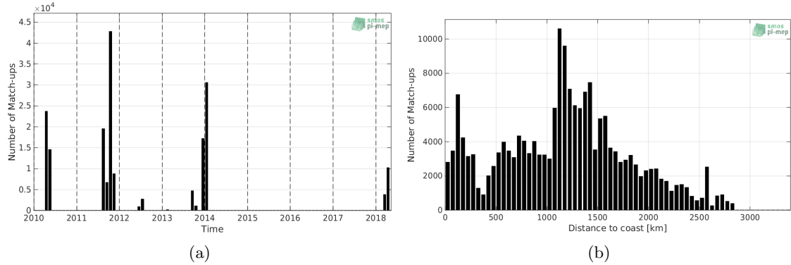
Figure 1: Number of match-ups between TSG-SAMOS and SMOS-L3-CATDS-CECOS-LOCEAN-V4-9DAYS-25KM SSS as a function of time (a) and as function of the distance to coast (b) over the South Atlantic Ocean Pi-MEP region and for the full satellite product period.
