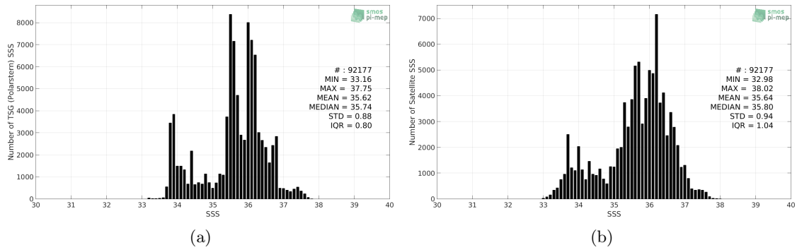
Figure 2: Histograms of SSS from TSG (Polarstern) (a) and SMOS SSS L3 v4 - 9 Days (CATDS-CECOS-LOCEAN) (b) considering all match-up pairs per bins of 0.1 over the South Atlantic Ocean Pi-MEP region and for the full satellite product period.
