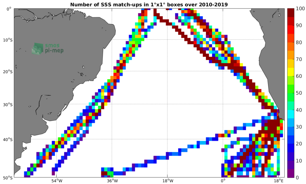
Figure 4: Number of SSS match-ups between TSG (Polarstern) SSS and the SMOS SSS L3 v4 - 9 Days (CATDS-CECOS-LOCEAN) SSS product for the South Atlantic Ocean Pi-MEP region over 1^\circ \times 1^\circ boxes and for the full satellite product period.
