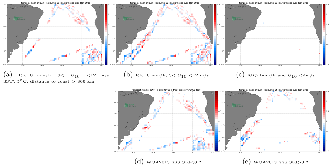
Figure 12: Temporal mean gridded over spatial boxes of size 1^\circ \times 1^\circ of \Delta SSS (SMOS SSS L3 v4 - 9 Days (CATDS-CECOS-LOCEAN) - TSG (Polarstern)) for 5 different subdatasets corresponding to: RR=0 mm/h, 3 < U_{10} < 12 m/s, SST > 5^\circ C , distance to coast > 800 km (a), RR=0 mm/h, 3 < U_{10} < 12 m/s (b), RR > 1 mm/h and U_{10} < 4 m/s (c), WOA2013 SSS Std < 0.2 (d), WOA2013 SSS Std > 0.2 (e).
