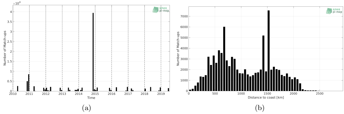
Figure 1: Number of match-ups between TSG (Polarstern) and SMOS SSS L3 v4 - 9 Days (CATDS-CECOS-LOCEAN) SSS as a function of time (a) and as function of the distance to coast (b) over the South Atlantic Ocean Pi-MEP region and for the full satellite product period.
