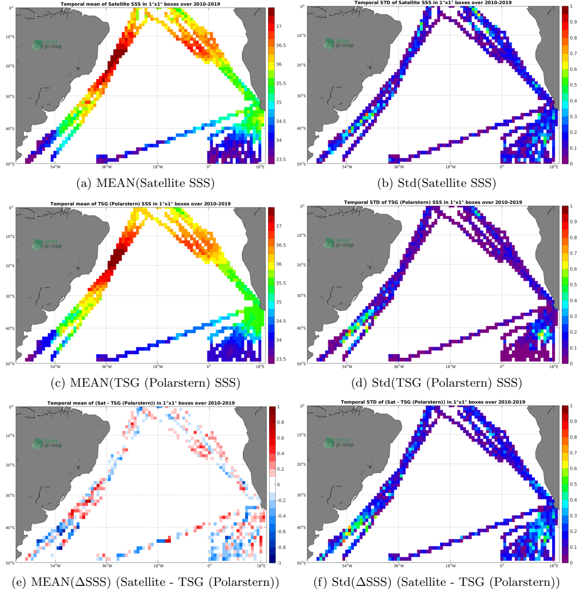
Figure 6: Temporal mean (left) and Std (right) of SSS from SMOS SSS L3 v4 - 9 Days (CATDS-CECOS-LOCEAN) (top), TSG (Polarstern) (middle), and of \Delta SSS (Satellite - TSG (Polarstern)). Only match-up pairs are used to generate these maps.
