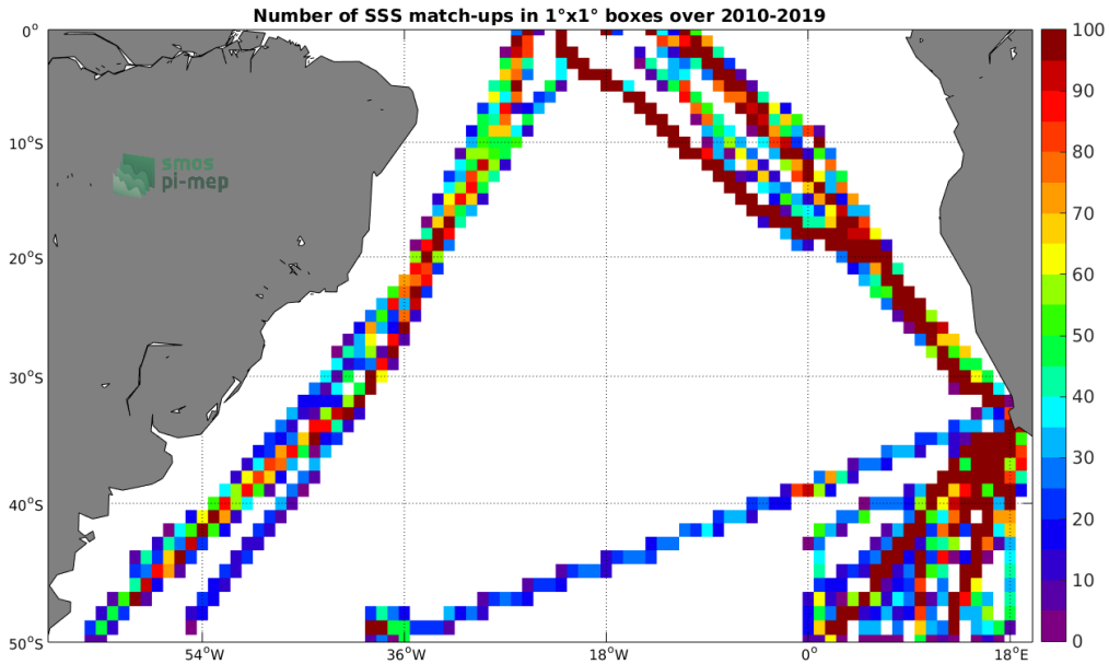
Figure 4: Number of SSS match-ups between TSG-POLARSTERN SSS and the SMOS-L3-CATDS-CECOS-LOCEAN-V4-9DAYS-25KM SSS product for the South Atlantic Ocean Pi-MEP region over 1°x1° boxes and for the full satellite product period.
