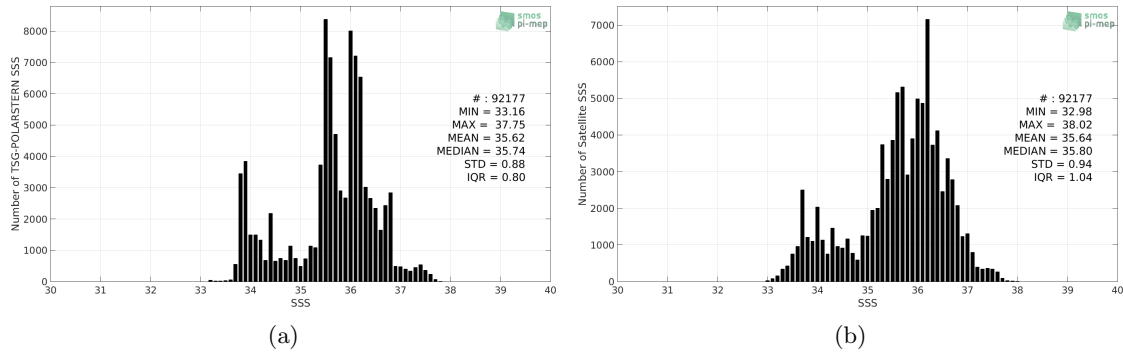
Figure 2: Histograms of SSS from TSG-POLARSTERN (a) and SMOS-L3-CATDS-CECOS-LOCEAN-V4-9DAYS-25KM (b) considering all match-up pairs per bins of 0.1 over the South Atlantic Ocean Pi-MEP region and for the full satellite product period.
