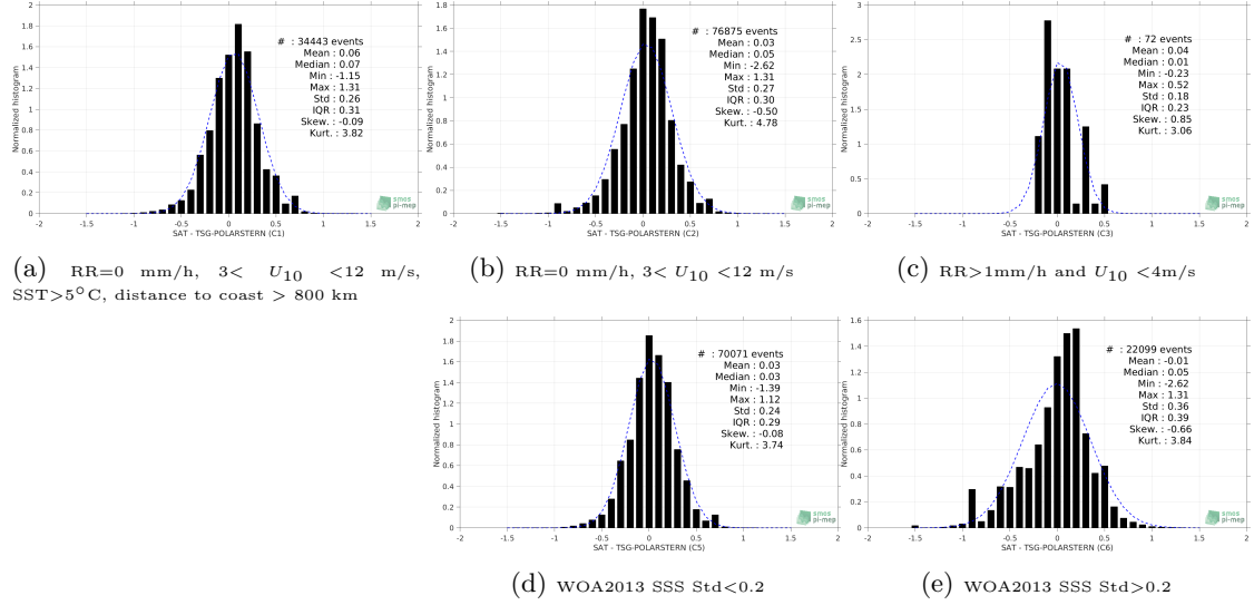
Figure 13: Normalized histogram of \Delta\text{SSS} (SMOS-L3-CATDS-CECOS-LOCEAN-V4-9DAYS-25KM - TSG-POLARSTERN) for 5 different subdatasets corresponding to: RR=0 mm/h, 3 < U_{10} < 12 m/s, SST > 5^\circ\text{C} , distance to coast > 800 km (a), RR=0 mm/h, 3 < U_{10} < 12 m/s (b), RR > 1\text{mm/h} and U_{10} < 4\text{m/s} (c), WOA2013 SSS Std < 0.2 (d), WOA2013 SSS Std > 0.2 (e).
