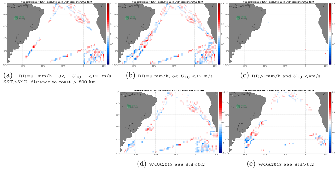
Figure 12: Temporal mean gridded over spatial boxes of size 1^\circ \times 1^\circ of \Delta SSS (SMOS-L3-CATDS-CECOS-LOCEAN-V4-9DAYS-25KM - TSG-POLARSTERN) for 5 different subdatasets corresponding to:RR=0 mm/h, 3 < U_{10} < 12 m/s, SST >5^\circ\text{C} , distance to coast > 800 km (a), RR=0 mm/h, 3 < U_{10} < 12 m/s (b), RR >1 mm/h and U_{10} < 4 m/s (c), WOA2013 SSS Std <0.2 (d), WOA2013 SSS Std >0.2 (e).
