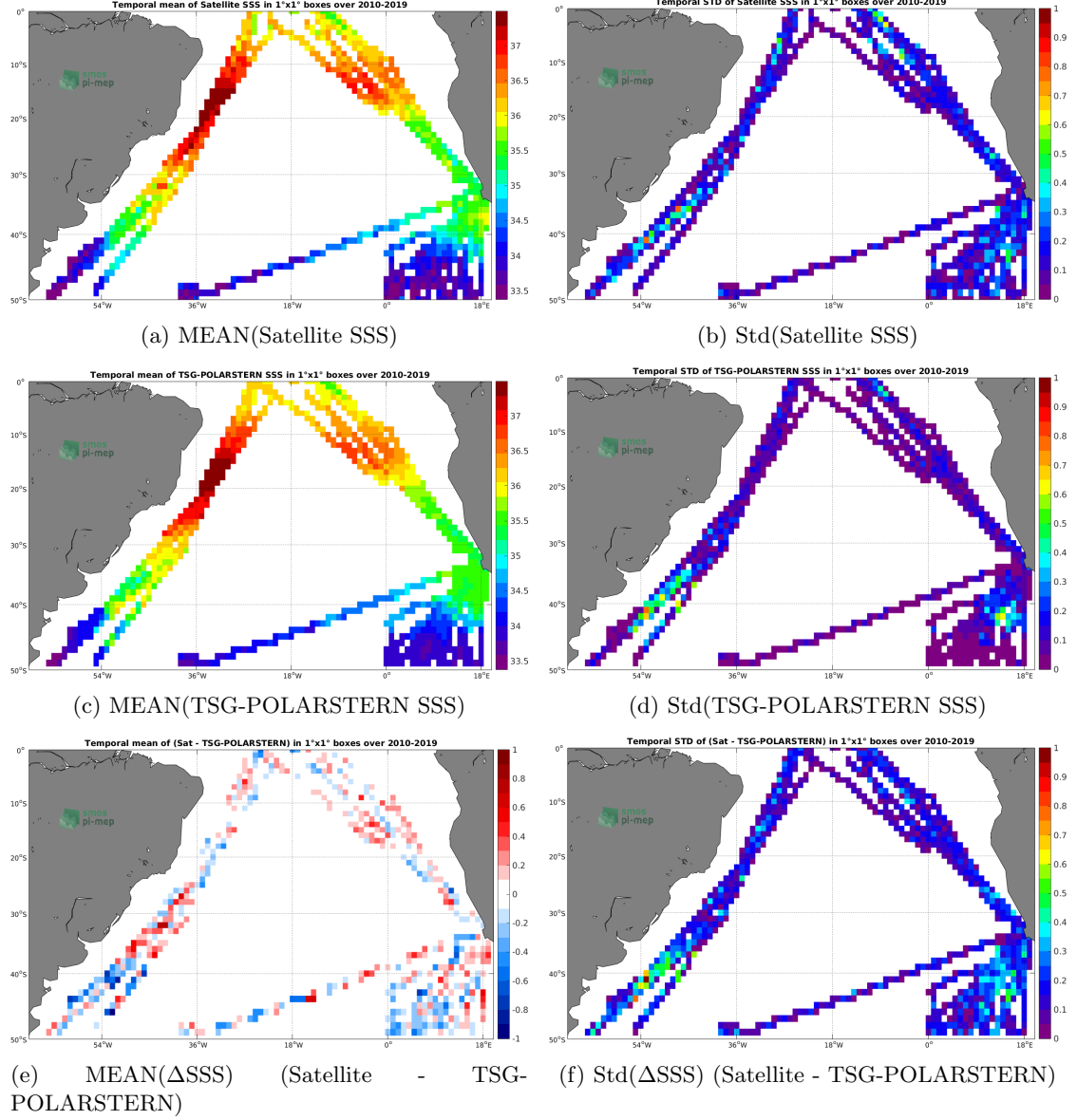
Figure 6: Temporal mean (left) and Std (right) of SSS from SMOS-L3-CATDS-CECOS-LOCEAN-V4-9DAYS-25KM (top), TSG-POLARSTERN (middle), and of \Delta SSS (Satellite - TSG-POLARSTERN). Only match-up pairs are used to generate these maps.
