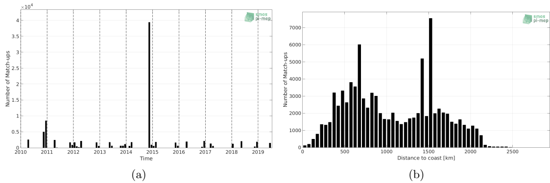
Figure 1: Number of match-ups between TSG-POLARSTERN and SMOS-L3-CATDS-CECOS-LOCEAN-V4-9DAYS-25KM SSS as a function of time (a) and as function of the distance to coast (b) over the South Atlantic Ocean Pi-MEP region and for the full satellite product period.
