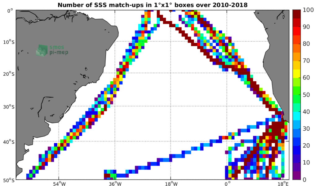
Figure 4: Number of SSS match-ups between TSG-POLARSTERN SSS and the SMOS-L3-CATDS-CECOS-LOCEAN-V4-9DAYS-25KM SSS product for the South Atlantic Ocean Pi-MEP region over 1^\circ \times 1^\circ boxes and for the full satellite product period.
