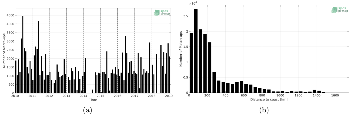
Figure 1: Number of match-ups between TSG-LEGOS-DM and SMOS-L3-CATDS-CECOS-LOCEAN-V4-9DAYS-25KM SSS as a function of time (a) and as function of the distance to coast (b) over the South Atlantic Ocean Pi-MEP region and for the full satellite product period.
