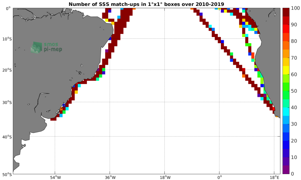
Figure 4: Number of SSS match-ups between TSG-LEGOS-DM SSS and the SMOS-L3-CATDS-CECOS-LOCEAN-V4-9DAYS-25KM SSS product for the South Atlantic Ocean Pi-MEP region over 1^\circ \times 1^\circ boxes and for the full satellite product period.
