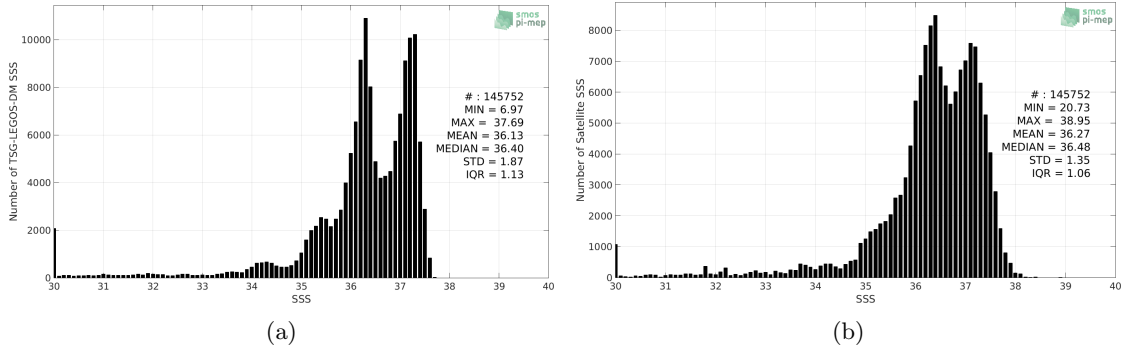
Figure 2: Histograms of SSS from TSG-LEGOS-DM (a) and SMOS-L3-CATDS-CECOS-LOCEAN-V4-9DAYS-25KM (b) considering all match-up pairs per bins of 0.1 over the South Atlantic Ocean Pi-MEP region and for the full satellite product period.
