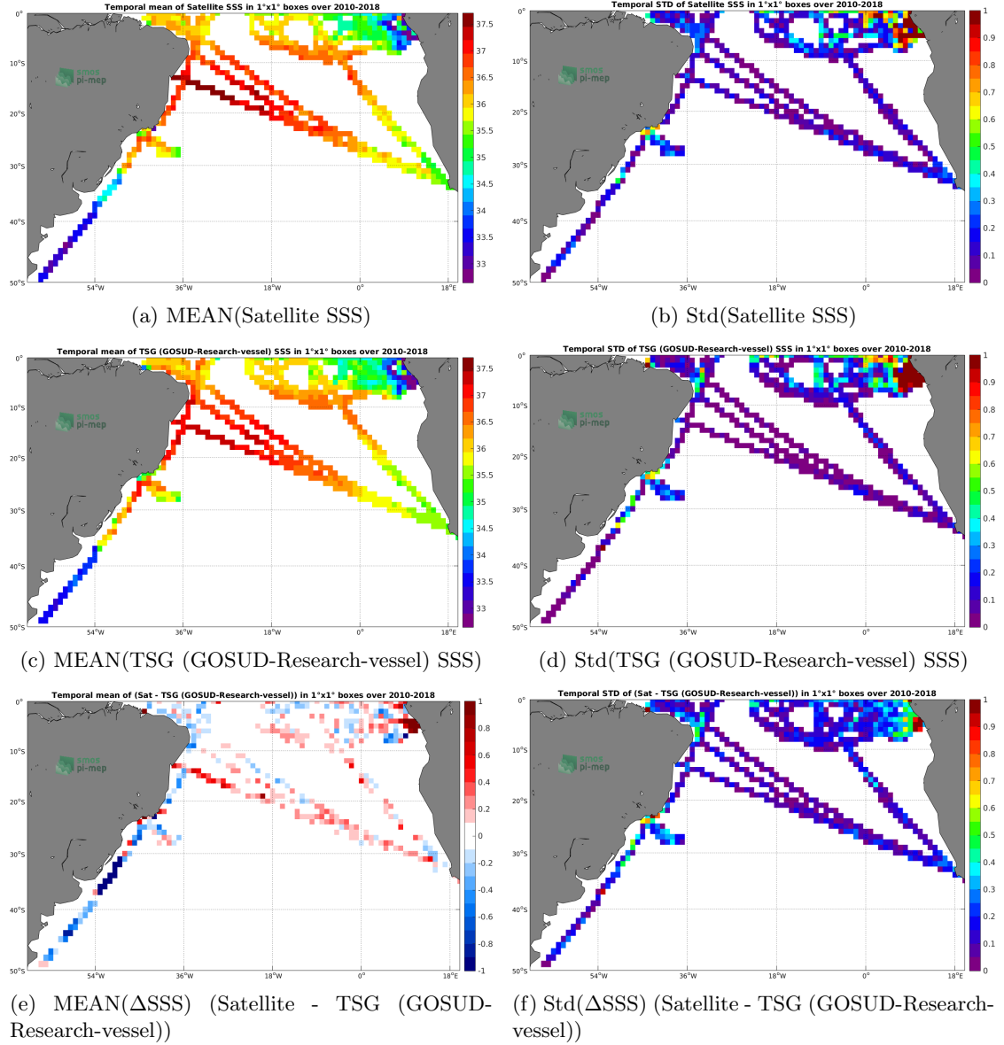
Figure 6: Temporal mean (left) and Std (right) of SSS from SMOS SSS L3 v4 - 9 Days (CATDS-CECOS-LOCEAN) (top), TSG (GOSUD-Research-vessel) (middle), and of \Delta SSS (Satellite - TSG (GOSUD-Research-vessel)). Only match-up pairs are used to generate these maps.
