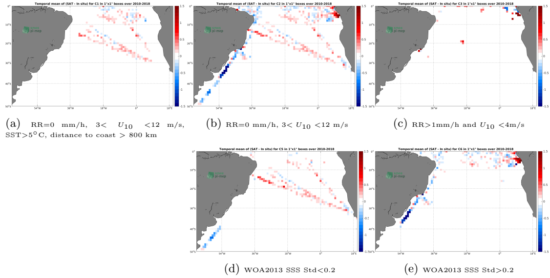
Figure 12: Temporal mean gridded over spatial boxes of size 1^\circ \times 1^\circ of \Delta SSS (SMOS SSS L3 v4 - 9 Days (CATDS-CECOS-LOCEAN) - TSG (GOSUD-Research-vessel)) for 5 different subdatasets corresponding to: RR=0 mm/h, 3 < U_{10} < 12 m/s, SST > 5^\circ C , distance to coast > 800 km (a), RR=0 mm/h, 3 < U_{10} < 12 m/s (b), RR > 1 mm/h and U_{10} < 4 m/s (c), WOA2013 SSS Std < 0.2 (d), WOA2013 SSS Std > 0.2 (e).
