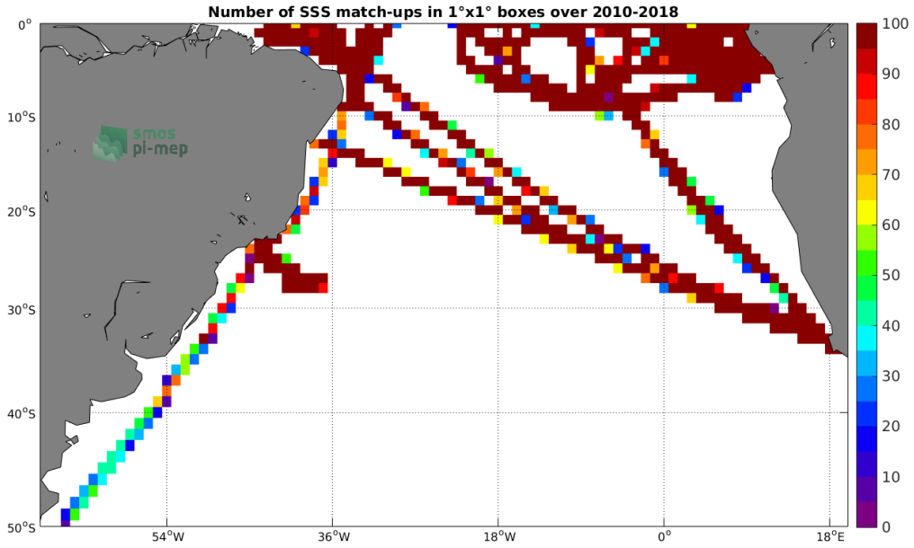
Figure 4: Number of SSS match-ups between TSG (GOSUD-Research-vessel) SSS and the SMOS SSS L3 v4 - 9 Days (CATDS-CECOS-LOCEAN) SSS product for the South Atlantic Ocean Pi-MEP region over 1^\circ \times 1^\circ boxes and for the full satellite product period.
