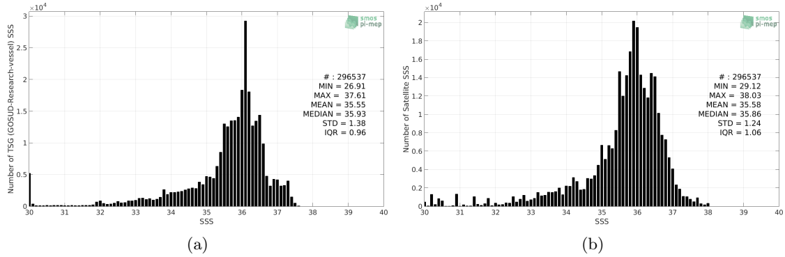
Figure 2: Histograms of SSS from TSG (GOSUD-Research-vessel) (a) and SMOS SSS L3 v4 - 9 Days (CATDS-CECOS-LOCEAN) (b) considering all match-up pairs per bins of 0.1 over the South Atlantic Ocean Pi-MEP region and for the full satellite product period.
