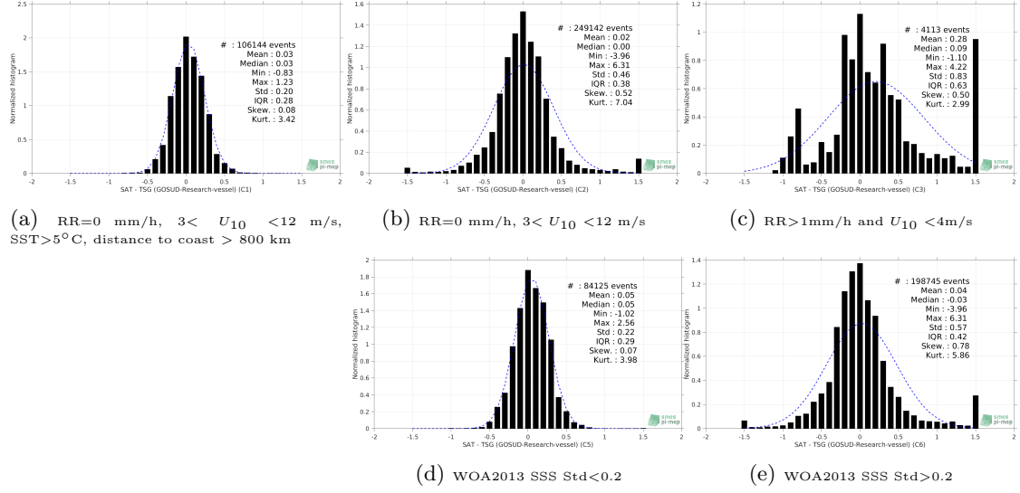
Figure 13: Normalized histogram of \Delta\text{SSS} (SMOS SSS L3 v4 - 9 Days (CATDS-CECOS-LOCEAN) - TSG (GOSUD-Research-vessel)) for 5 different subdatasets corresponding to: RR=0 mm/h, 3 < U_{10} < 12 m/s, SST > 5^\circ\text{C} , distance to coast > 800 km (a), RR=0 mm/h, 3 < U_{10} < 12 m/s (b), RR > 1\text{mm/h} and U_{10} < 4\text{m/s} (c), WOA2013 SSS Std < 0.2 (d), WOA2013 SSS Std > 0.2 (e).
