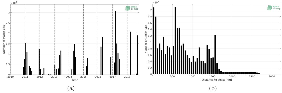
Figure 1: Number of match-ups between TSG-GOSUD-Research-vessel and SMOS-L3-CATDS-CECOS-LOCEAN-V4-9DAYS-25KM SSS as a function of time (a) and as function of the distance to coast (b) over the South Atlantic Ocean Pi-MEP region and for the full satellite product period.
