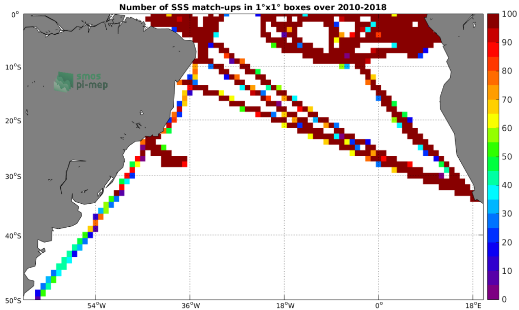
Figure 4: Number of SSS match-ups between TSG-GOSUD-Research-vessel SSS and the SMOS-L3-CATDS-CECOS-LOCEAN-V4-9DAYS-25KM SSS product for the South Atlantic Ocean Pi-MEP region over 1^\circ \times 1^\circ boxes and for the full satellite product period.
