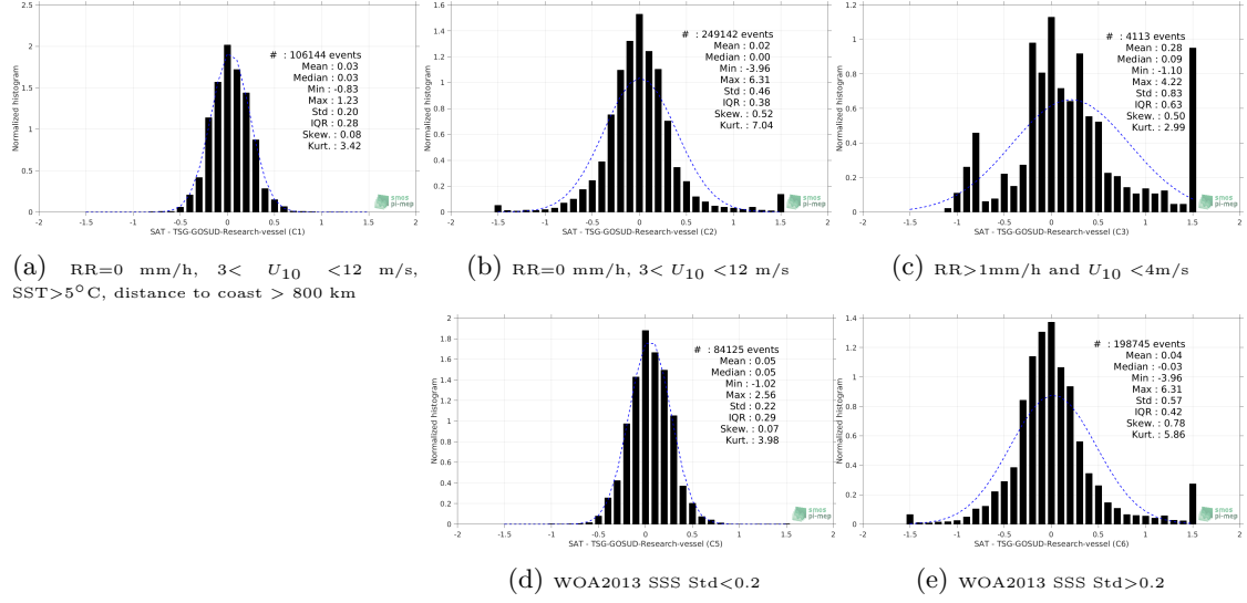
Figure 13: Normalized histogram of \Delta SSS (SMOS-L3-CATDS-CECOS-LOCEAN-V4-9DAYS-25KM - TSG-GOSUD-Research-vessel) for 5 different subdatasets corresponding to: RR=0 mm/h, 3 < U_{10} < 12 m/s, SST > 5°C, distance to coast > 800 km (a), RR=0 mm/h, 3 < U_{10} < 12 m/s (b), RR > 1 mm/h and U_{10} < 4 m/s (c), WOA2013 SSS Std < 0.2 (d), WOA2013 SSS Std > 0.2 (e).
