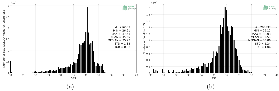
Figure 2: Histograms of SSS from TSG-GOSUD-Research-vessel (a) and SMOS-L3-CATDS-CECOS-LOCEAN-V4-9DAYS-25KM (b) considering all match-up pairs per bins of 0.1 over the South Atlantic Ocean Pi-MEP region and for the full satellite product period.
