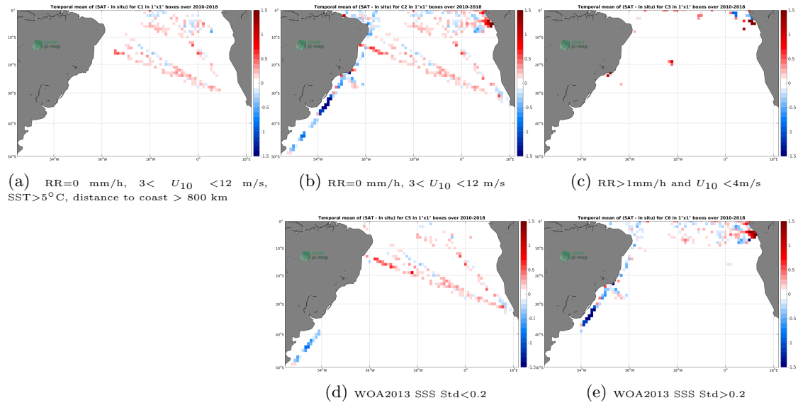
Figure 12: Temporal mean gridded over spatial boxes of size 1^\circ \times 1^\circ of \Delta SSS (SMOS-L3-CATDS-CECOS-LOCEAN-V4-9DAYS-25KM - TSG-GOSUD-Research-vessel) for 5 different subdatasets corresponding to:RR=0 mm/h, 3 < U_{10} < 12 m/s, SST >5^\circ\text{C} , distance to coast > 800 km (a), RR=0 mm/h, 3 < U_{10} < 12 m/s (b), RR >1 mm/h and U_{10} < 4 m/s (c), WOA2013 SSS Std <0.2 (d), WOA2013 SSS Std >0.2 (e).
