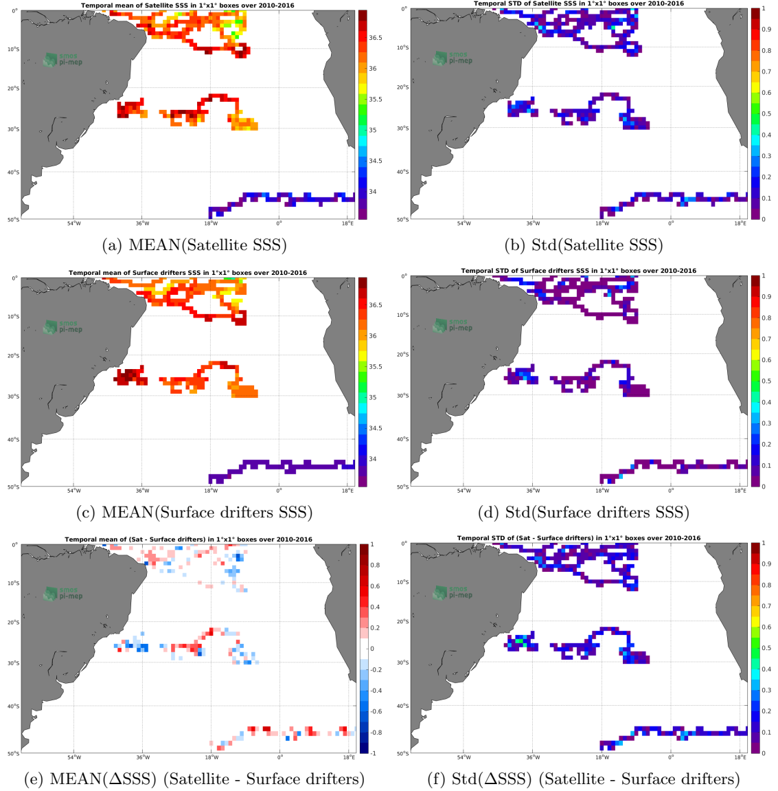
Figure 5: Temporal mean (left) and Std (right) of SSS from SMOS SSS L3 v4 - 9 Days (CATDS-CECOS-LOCEAN) (top), Surface drifters (middle), and of \Delta SSS (Satellite - Surface drifters). Only match-up pairs are used to generate these maps.
