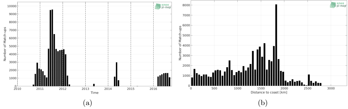
Figure 1: Number of match-ups between Surface drifters and SMOS SSS L3 v4 - 9 Days (CATDS-CECOS-LOCEAN) SSS as a function of time (a) and as function of the distance to coast (b) over the South Atlantic Ocean Pi-MEP region and for the full satellite product period.
