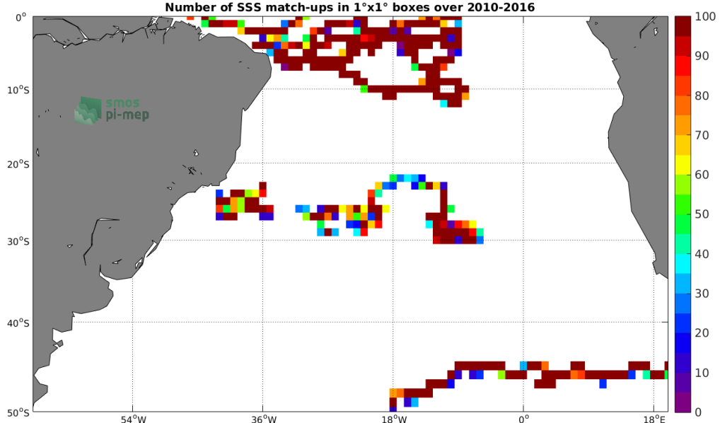
Figure 3: Number of SSS match-ups between Surface drifters SSS and the SMOS SSS L3 v4 - 9 Days (CATDS-CECOS-LOCEAN) SSS product for the South Atlantic Ocean Pi-MEP region over 1^\circ \times 1^\circ boxes and for the full satellite product period.
