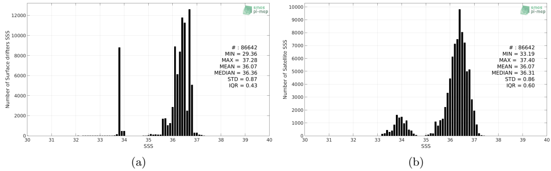
Figure 2: Histograms of SSS from Surface drifters (a) and SMOS SSS L3 v4 - 9 Days (CATDS-CECOS-LOCEAN) (b) considering all match-up pairs per bins of 0.1 over the South Atlantic Ocean Pi-MEP region and for the full satellite product period.
