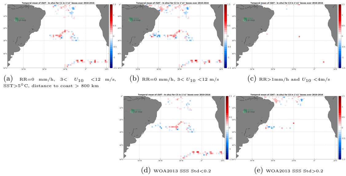
Figure 11: Temporal mean gridded over spatial boxes of size 1^\circ \times 1^\circ of \Delta SSS (SMOS SSS L3 v4 - 9 Days (CATDS-CECOS-LOCEAN) - Surface drifters) for 5 different subdatasets corresponding to: RR=0 mm/h, 3 < U_{10} < 12 m/s, SST > 5^\circ C , distance to coast > 800 km (a), RR=0 mm/h, 3 < U_{10} < 12 m/s (b), RR > 1 mm/h and U_{10} < 4 m/s (c), WOA2013 SSS Std < 0.2 (d), WOA2013 SSS Std > 0.2 (e).
