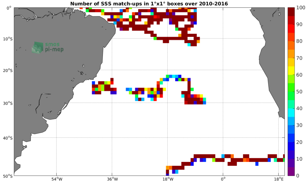
Figure 3: Number of SSS match-ups between Surface drifters SSS and the SMOS-L3-CATDS-CECOS-LOCEAN-V4-9DAYS-25KM SSS product for the South Atlantic Ocean Pi-MEP region over 1^\circ \times 1^\circ boxes and for the full satellite product period.
