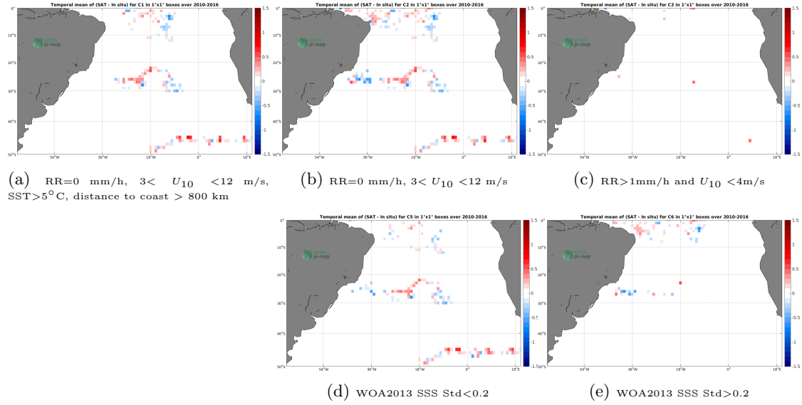
Figure 11: Temporal mean gridded over spatial boxes of size 1^\circ \times 1^\circ of \Delta SSS (SMOS-L3-CATDS-CECOS-LOCEAN-V4-9DAYS-25KM - Surface drifters) for 5 different subdatasets corresponding to: RR=0 mm/h, 3 < U_{10} < 12 m/s, SST > 5^\circ C , distance to coast > 800 km (a), RR=0 mm/h, 3 < U_{10} < 12 m/s (b), RR > 1 mm/h and U_{10} < 4 m/s (c), WOA2013 SSS Std < 0.2 (d), WOA2013 SSS Std > 0.2 (e).
