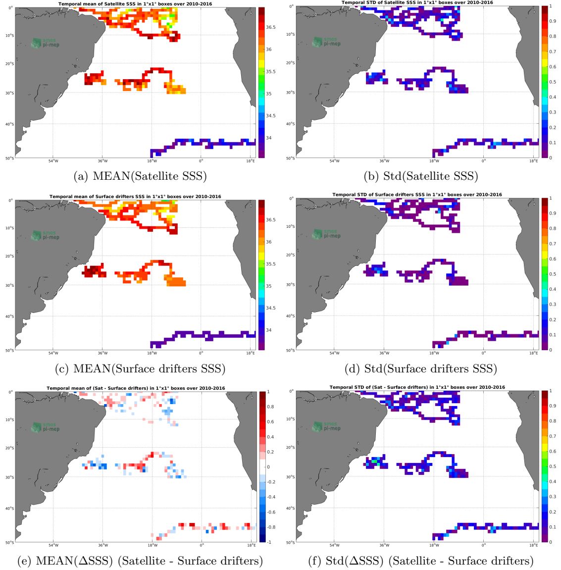
Figure 5: Temporal mean (left) and Std (right) of SSS from SMOS-L3-CATDS-CECOS-LOCEAN-V4-9DAYS-25KM (top), Surface drifters (middle), and of \Delta SSS (Satellite - Surface drifters). Only match-up pairs are used to generate these maps.
