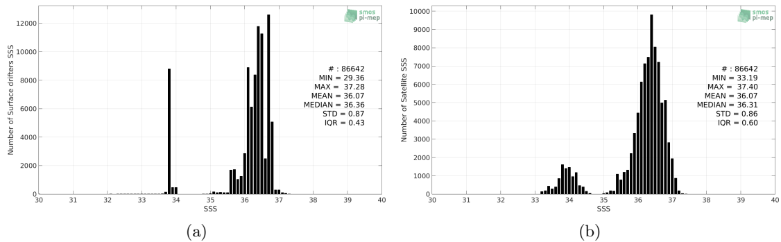
Figure 2: Histograms of SSS from Surface drifters (a) and SMOS-L3-CATDS-CECOS-LOCEAN-V4-9DAYS-25KM (b) considering all match-up pairs per bins of 0.1 over the South Atlantic Ocean Pi-MEP region and for the full satellite product period.
