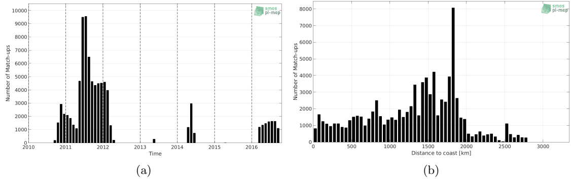
Figure 1: Number of match-ups between Surface drifters and SMOS-L3-CATDS-CECOS-LOCEAN-V4-9DAYS-25KM SSS as a function of time (a) and as function of the distance to coast (b) over the South Atlantic Ocean Pi-MEP region and for the full satellite product period.
