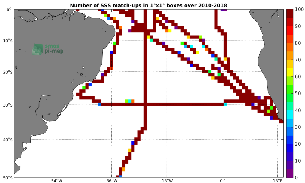
Figure 4: Number of SSS match-ups between TSG (SAMOS) SSS and the SMOS SSS L3 v4 - 18 Days (CATDS-CECOS-LOCEAN) SSS product for the South Atlantic Ocean Pi-MEP region over 1^\circ \times 1^\circ boxes and for the full satellite product period.
