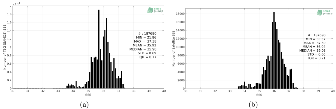
Figure 2: Histograms of SSS from TSG (SAMOS) (a) and SMOS SSS L3 v4 - 18 Days (CATDS-CECOS-LOCEAN) (b) considering all match-up pairs per bins of 0.1 over the South Atlantic Ocean Pi-MEP region and for the full satellite product period.
