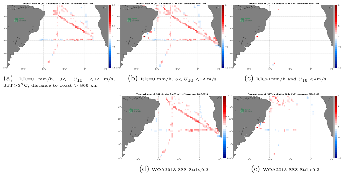
Figure 12: Temporal mean gridded over spatial boxes of size 1^\circ \times 1^\circ of \Delta SSS (SMOS SSS L3 v4 - 18 Days (CATDS-CECOS-LOCEAN) - TSG (SAMOS)) for 5 different subdatasets corresponding to: RR=0 mm/h, 3 < U_{10} < 12 m/s, SST > 5^\circ\text{C} , distance to coast > 800 km (a), RR=0 mm/h, 3 < U_{10} < 12 m/s (b), RR > 1 mm/h and U_{10} < 4 m/s (c), WOA2013 SSS Std < 0.2 (d), WOA2013 SSS Std > 0.2 (e).
