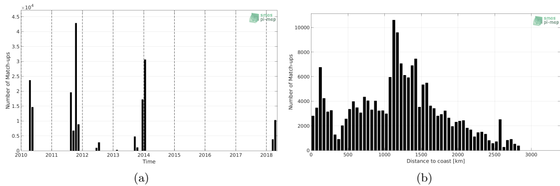
Figure 1: Number of match-ups between TSG (SAMOS) and SMOS SSS L3 v4 - 18 Days (CATDS-CECOS-LOCEAN) SSS as a function of time (a) and as function of the distance to coast (b) over the South Atlantic Ocean Pi-MEP region and for the full satellite product period.
