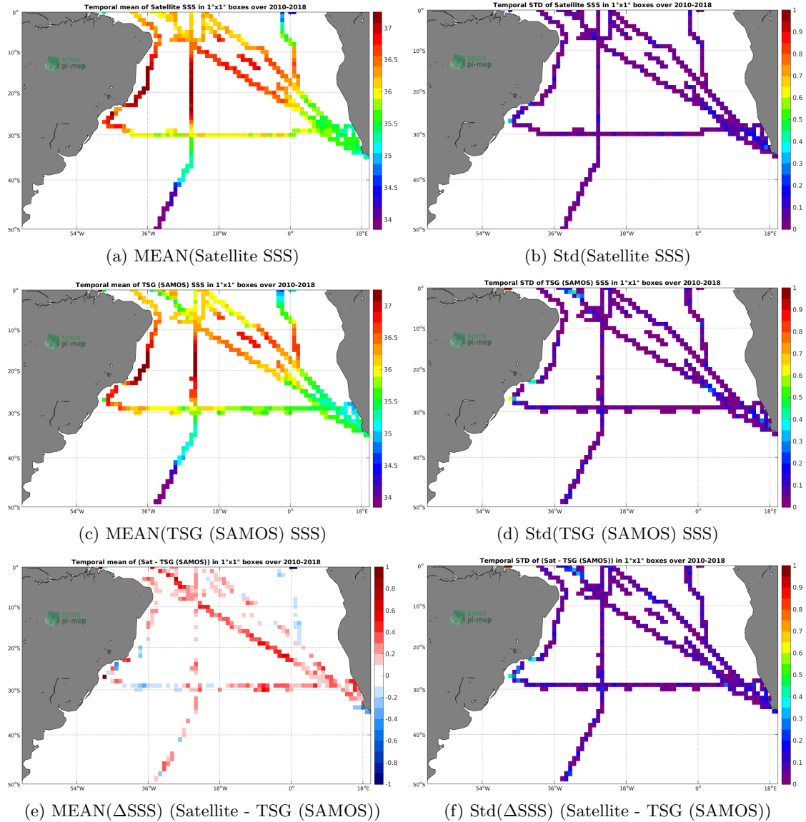
Figure 6: Temporal mean (left) and Std (right) of SSS from SMOS SSS L3 v4 - 18 Days (CATDS-CECOS-LOCEAN) (top), TSG (SAMOS) (middle), and of \Delta SSS (Satellite - TSG (SAMOS)). Only match-up pairs are used to generate these maps.
