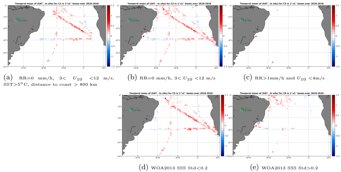
Figure 12: Temporal mean gridded over spatial boxes of size 1^\circ \times 1^\circ of \Delta SSS (SMOS-L3-CATDS-CECOS-LOCEAN-V4-18DAYS-25KM - TSG-SAMOS) for 5 different subdatasets corresponding to:RR=0 mm/h, 3 < U_{10} < 12 m/s, SST >5^\circ\text{C} , distance to coast > 800 km (a), RR=0 mm/h, 3 < U_{10} < 12 m/s (b), RR >1 mm/h and U_{10} < 4 m/s (c), WOA2013 SSS Std <0.2 (d), WOA2013 SSS Std >0.2 (e).
