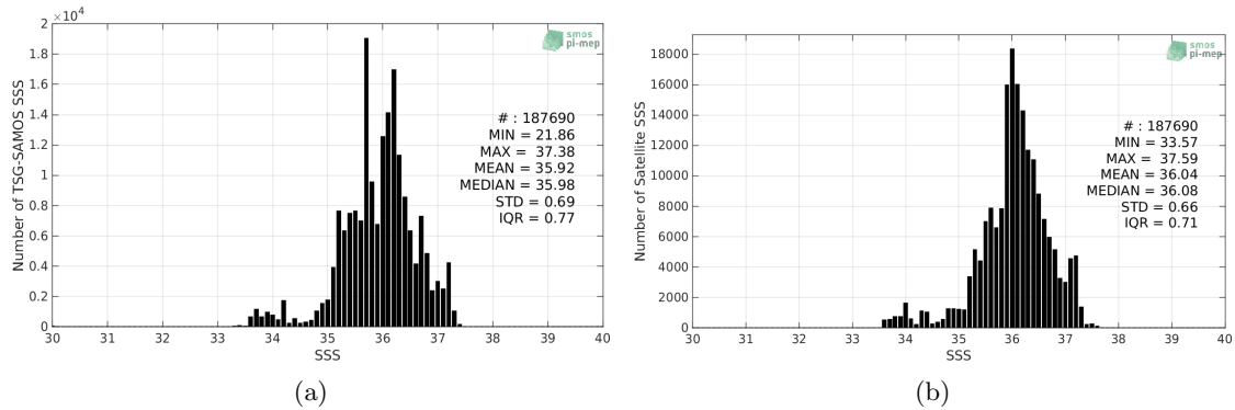
Figure 2: Histograms of SSS from TSG-SAMOS (a) and SMOS-L3-CATDS-CECOS-LOCEAN-V4-18DAYS-25KM (b) considering all match-up pairs per bins of 0.1 over the South Atlantic Ocean Pi-MEP region and for the full satellite product period.
