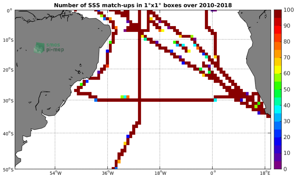
Figure 4: Number of SSS match-ups between TSG-SAMOS SSS and the SMOS-L3-CATDS-CECOS-LOCEAN-V4-18DAYS-25KM SSS product for the South Atlantic Ocean Pi-MEP region over 1^\circ \times 1^\circ boxes and for the full satellite product period.
