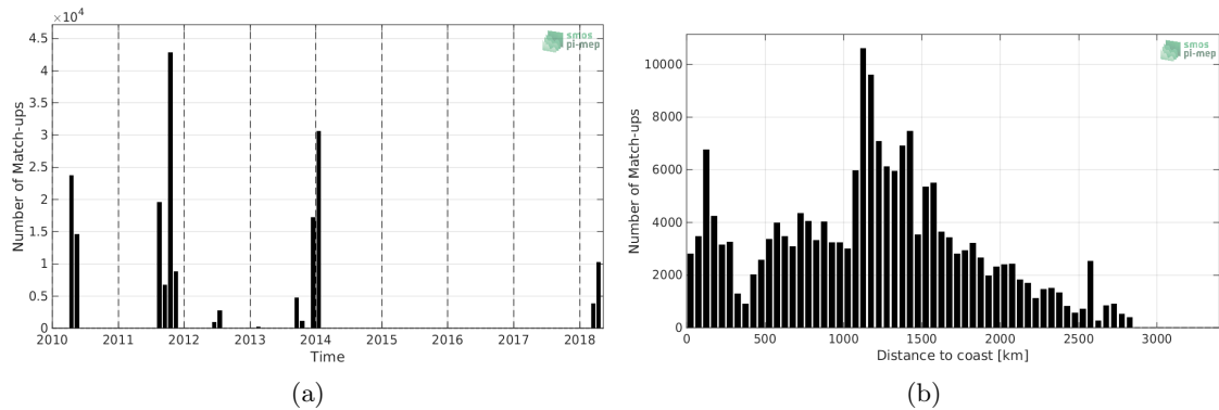
Figure 1: Number of match-ups between TSG-SAMOS and SMOS-L3-CATDS-CECOS-LOCEAN-V4-18DAYS-25KM SSS as a function of time (a) and as function of the distance to coast (b) over the South Atlantic Ocean Pi-MEP region and for the full satellite product period.
