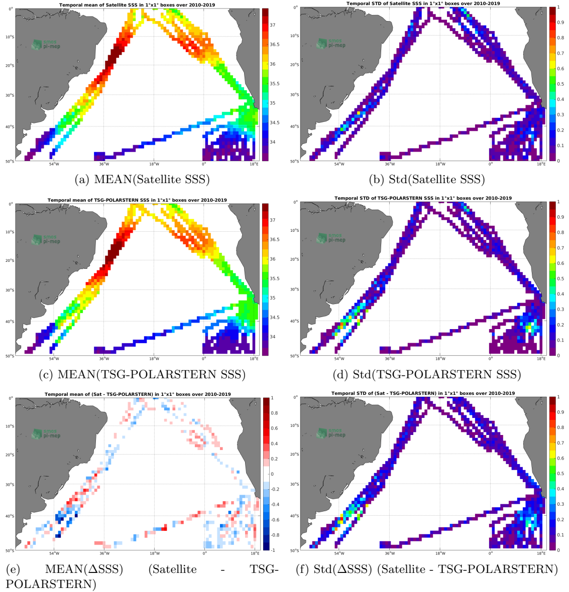
Figure 6: Temporal mean (left) and Std (right) of SSS from SMOS-L3-CATDS-CECOS-LOCEAN-V4-18DAYS-25KM (top), TSG-POLARSTERN (middle), and of \Delta SSS (Satellite - TSG-POLARSTERN). Only match-up pairs are used to generate these maps.
