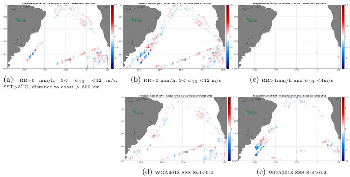
Figure 12: Temporal mean gridded over spatial boxes of size 1^\circ \times 1^\circ of \Delta SSS (SMOS-L3-CATDS-CECOS-LOCEAN-V4-18DAYS-25KM - TSG-POLARSTERN) for 5 different subdatasets corresponding to:RR=0 mm/h, 3 < U_{10} < 12 m/s, SST >5^\circ C, distance to coast > 800 km (a), RR=0 mm/h, 3 < U_{10} < 12 m/s (b), RR >1 mm/h and U_{10} < 4 m/s (c), WOA2013 SSS Std <0.2 (d), WOA2013 SSS Std >0.2 (e).
