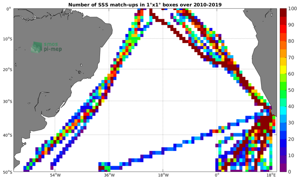
Figure 4: Number of SSS match-ups between TSG-POLARSTERN SSS and the SMOS-L3-CATDS-CECOS-LOCEAN-V4-18DAYS-25KM SSS product for the South Atlantic Ocean Pi-MEP region over 1^\circ \times 1^\circ boxes and for the full satellite product period.
