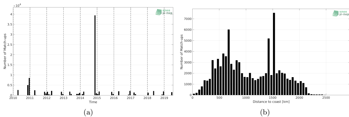
Figure 1: Number of match-ups between TSG-POLARSTERN and SMOS-L3-CATDS-CECOS-LOCEAN-V4-18DAYS-25KM SSS as a function of time (a) and as function of the distance to coast (b) over the South Atlantic Ocean Pi-MEP region and for the full satellite product period.
