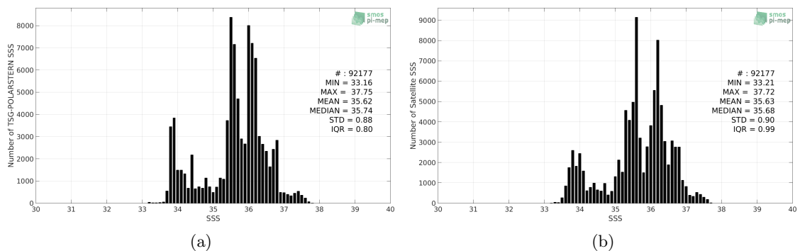
Figure 2: Histograms of SSS from TSG-POLARSTERN (a) and SMOS-L3-CATDS-CECOS-LOCEAN-V4-18DAYS-25KM (b) considering all match-up pairs per bins of 0.1 over the South Atlantic Ocean Pi-MEP region and for the full satellite product period.
