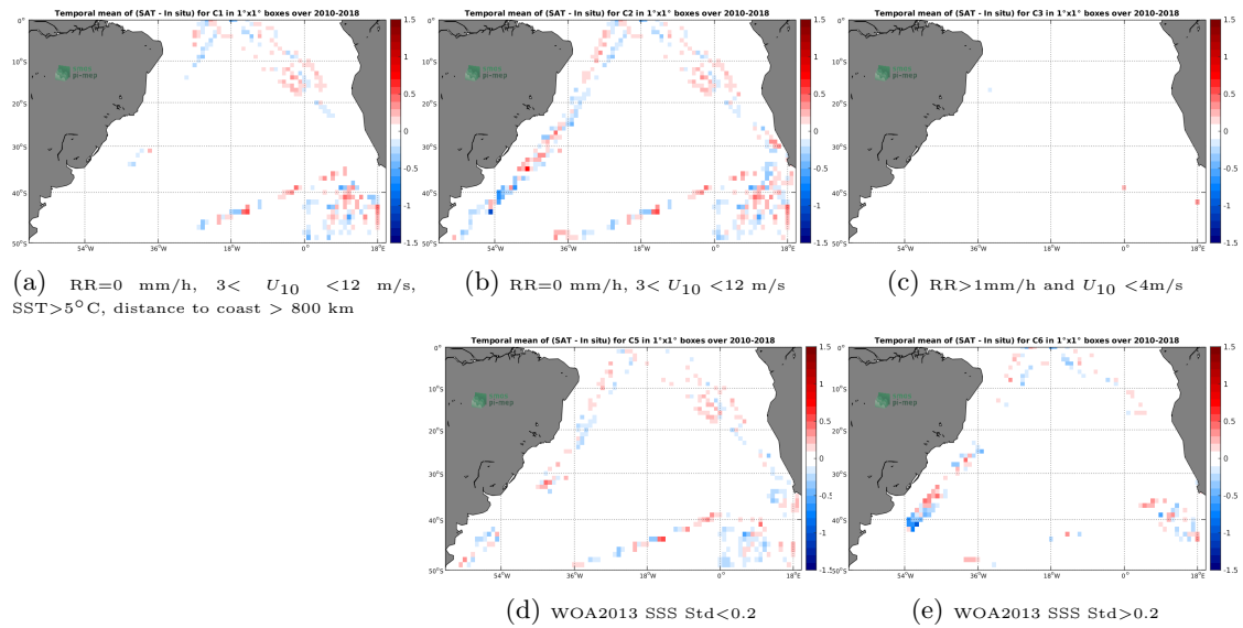
Figure 12: Temporal mean gridded over spatial boxes of size 1^\circ \times 1^\circ of \Delta\text{SSS} (SMOS-L3-CATDS-CECOS-LOCEAN-V4-18DAYS-25KM - TSG-POLARSTERN) for 5 different subdatasets corresponding to:RR=0 mm/h, 3 < U_{10} < 12 m/s, SST >5^\circ\text{C} , distance to coast > 800 km (a), RR=0 mm/h, 3 < U_{10} < 12 m/s (b), RR >1 mm/h and U_{10} < 4 m/s (c), WOA2013 SSS Std <0.2 (d), WOA2013 SSS Std >0.2 (e).
