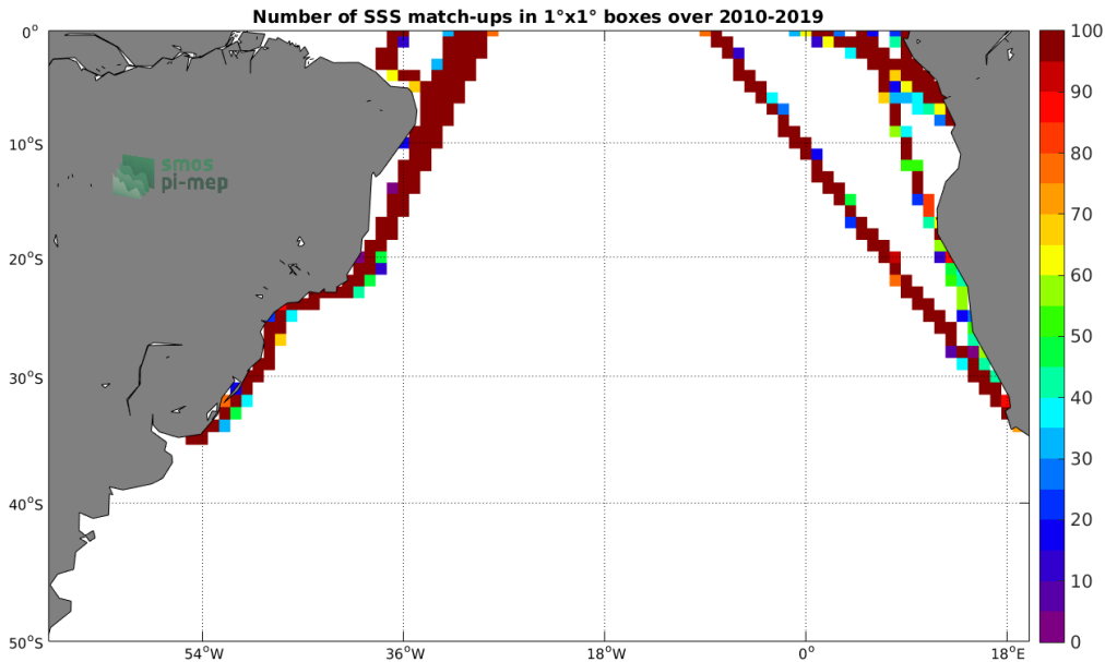
Figure 4: Number of SSS match-ups between TSG (LEGOS-DM) SSS and the SMOS SSS L3 v4 - 18 Days (CATDS-CECOS-LOCEAN) SSS product for the South Atlantic Ocean Pi-MEP region over 1^\circ \times 1^\circ boxes and for the full satellite product period.
