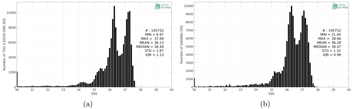
Figure 2: Histograms of SSS from TSG (LEGOS-DM) (a) and SMOS SSS L3 v4 - 18 Days (CATDS-CECOS-LOCEAN) (b) considering all match-up pairs per bins of 0.1 over the South Atlantic Ocean Pi-MEP region and for the full satellite product period.
