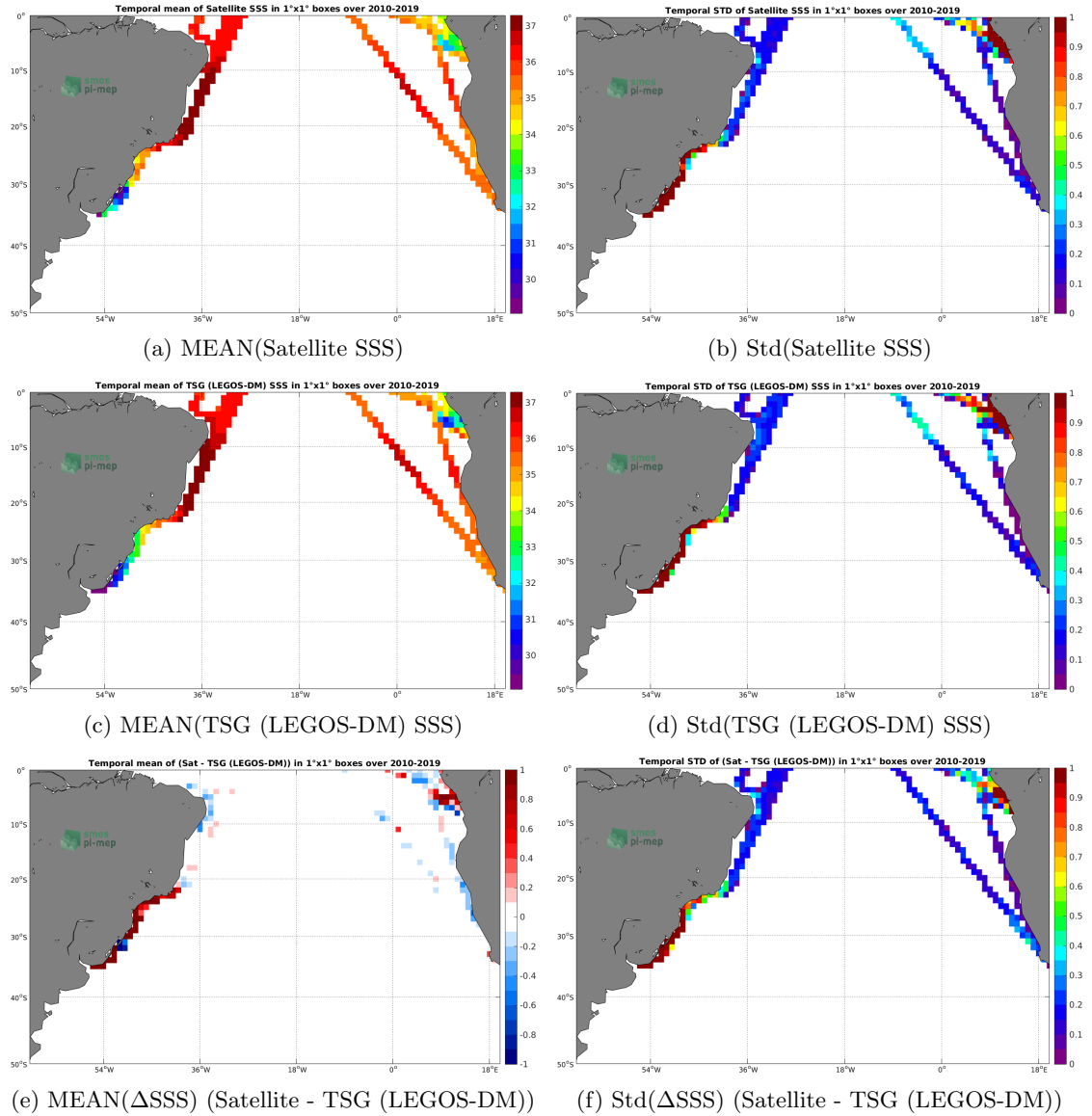
Figure 6: Temporal mean (left) and Std (right) of SSS from SMOS SSS L3 v4 - 18 Days (CATDS-CECOS-LOCEAN) (top), TSG (LEGOS-DM) ( in situ ) dataset (middle), and of \Delta SSS (Satellite - TSG (LEGOS-DM)). Only match-up pairs are used to generate these maps.
