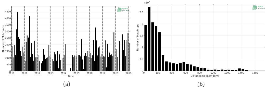
Figure 1: Number of match-ups between TSG (LEGOS-DM) and SMOS SSS L3 v4 - 18 Days (CATDS-CECOS-LOCEAN) SSS as a function of time (a) and as function of the distance to coast (b) over the South Atlantic Ocean Pi-MEP region and for the full satellite product period.
