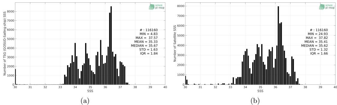
Figure 2: Histograms of SSS from TSG (GOSUD-Sailing-ship) (a) and SMOS SSS L3 v4 - 18 Days (CATDS-CECOS-LOCEAN) (b) considering all match-up pairs per bins of 0.1 over the South Atlantic Ocean Pi-MEP region and for the full satellite product period.
