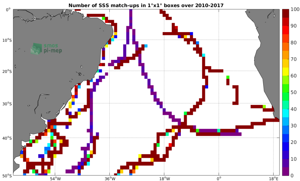
Figure 4: Number of SSS match-ups between TSG (GOSUD-Sailing-ship) SSS and the SMOS SSS L3 v4 - 18 Days (CATDS-CECOS-LOCEAN) SSS product for the South Atlantic Ocean Pi-MEP region over 1^\circ \times 1^\circ boxes and for the full satellite product period.
