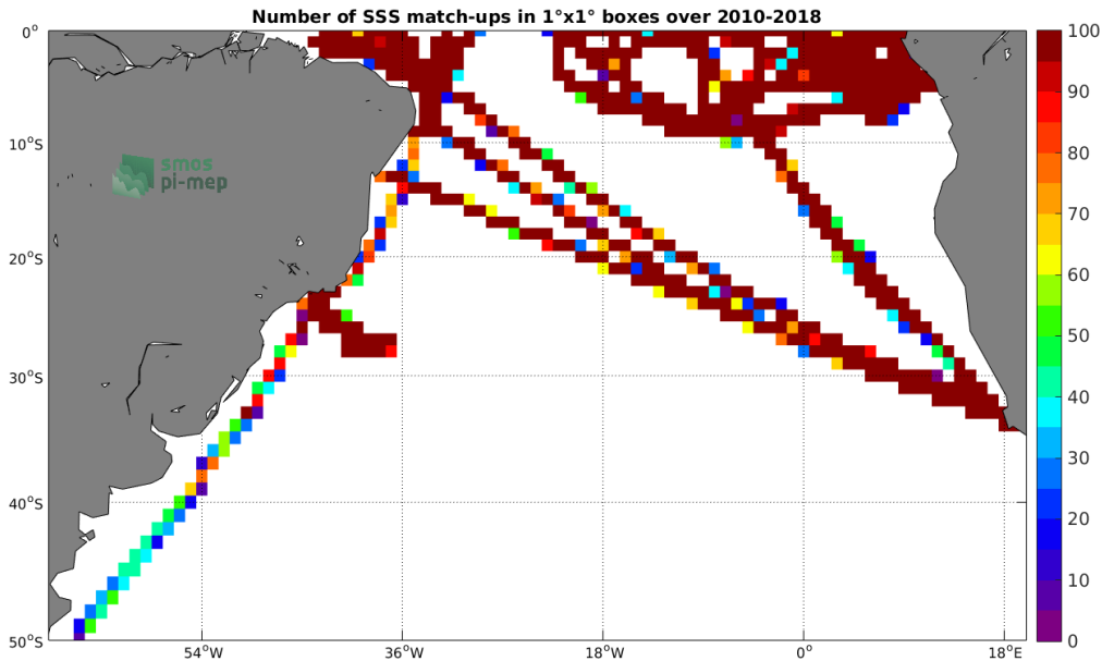
Figure 4: Number of SSS match-ups between TSG (GOSUD-Research-vessel) SSS and the SMOS SSS L3 v4 - 18 Days (CATDS-CECOS-LOCEAN) SSS product for the South Atlantic Ocean Pi-MEP region over 1°x1° boxes and for the full satellite product period.
