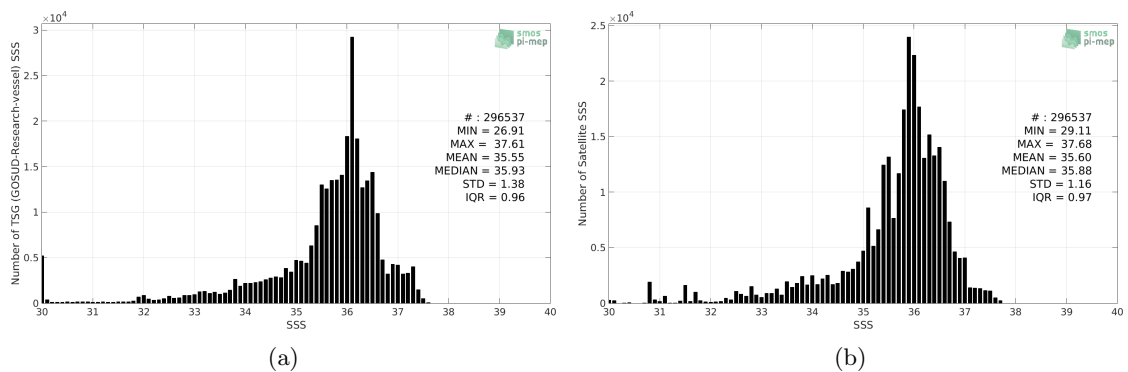
Figure 2: Histograms of SSS from TSG (GOSUD-Research-vessel) (a) and SMOS SSS L3 v4 - 18 Days (CATDS-CECOS-LOCEAN) (b) considering all match-up pairs per bins of 0.1 over the South Atlantic Ocean Pi-MEP region and for the full satellite product period.
