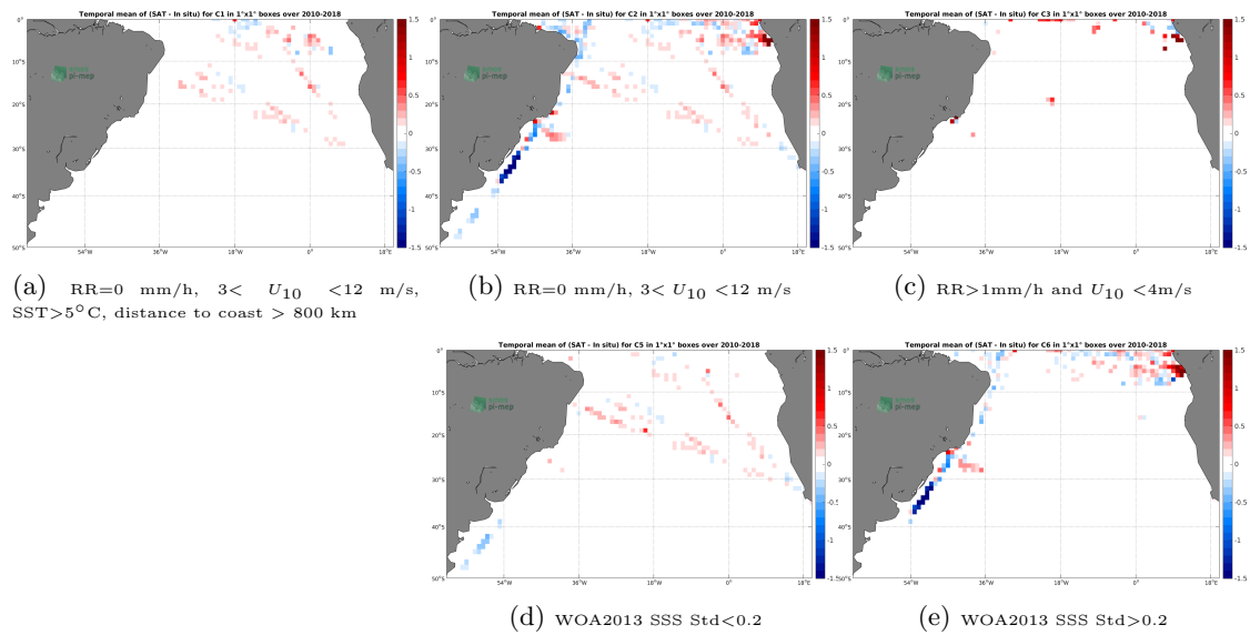
Figure 12: Temporal mean gridded over spatial boxes of size 1^\circ \times 1^\circ of \Delta SSS (SMOS SSS L3 v4 - 18 Days (CATDS-CECOS-LOCEAN) - TSG (GOSUD-Research-vessel)) for 5 different subdatasets corresponding to: RR=0 mm/h, 3 < U_{10} < 12 m/s, SST > 5°C, distance to coast > 800 km (a), RR=0 mm/h, 3 < U_{10} < 12 m/s (b), RR > 1mm/h and U_{10} < 4 m/s (c), WOA2013 SSS Std < 0.2 (d), WOA2013 SSS Std > 0.2 (e).
