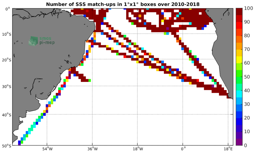
Figure 4: Number of SSS match-ups between TSG-GOSUD-Research-vessel SSS and the SMOS-L3-CATDS-CECOS-LOCEAN-V4-18DAYS-25KM SSS product for the South Atlantic Ocean Pi-MEP region over 1^\circ \times 1^\circ boxes and for the full satellite product period.
