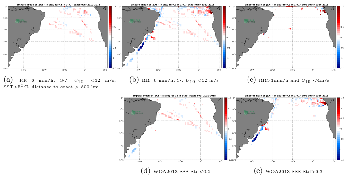
Figure 12: Temporal mean gridded over spatial boxes of size 1^\circ \times 1^\circ of \Delta SSS (SMOS-L3-CATDS-CECOS-LOCEAN-V4-18DAYS-25KM - TSG-GOSUD-Research-vessel) for 5 different subdatasets corresponding to:RR=0 mm/h, 3 < U_{10} < 12 m/s, SST >5^\circ\text{C} , distance to coast > 800 km (a), RR=0 mm/h, 3 < U_{10} < 12 m/s (b), RR >1 mm/h and U_{10} < 4 m/s (c), WOA2013 SSS Std <0.2 (d), WOA2013 SSS Std >0.2 (e).
