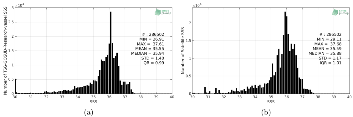
Figure 2: Histograms of SSS from TSG-GOSUD-Research-vessel (a) and SMOS-L3-CATDS-CECOS-LOCEAN-V4-18DAYS-25KM (b) considering all match-up pairs per bins of 0.1 over the South Atlantic Ocean Pi-MEP region and for the full satellite product period.
