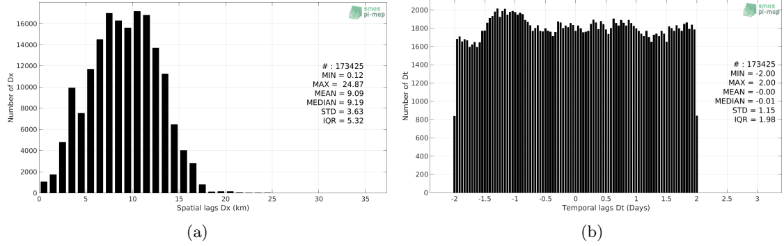
Figure 5: Histograms of the spatial (a) and temporal (b) lags between the time of the TSG-SAMOS measurements and the date of the corresponding SMOS-L3-CATDS-CECOS-LOCEAN-V3-9DAYS-25KM SSS product.
