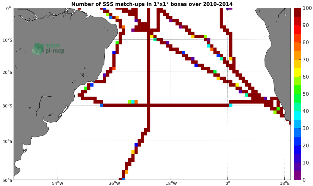
Figure 4: Number of SSS match-ups between TSG-SAMOS SSS and the SMOS-L3-CATDS-CECOS-LOCEAN-V3-9DAYS-25KM SSS product for the South Atlantic Ocean Pi-MEP region over 1°x1° boxes and for the full satellite product period.
