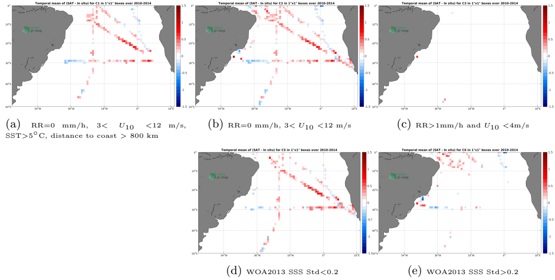
Figure 12: Temporal mean gridded over spatial boxes of size 1^\circ \times 1^\circ of \Delta SSS (SMOS-L3-CATDS-CECOS-LOCEAN-V3-9DAYS-25KM - TSG-SAMOS) for 5 different subdatasets corresponding to: RR=0 mm/h, 3 < U_{10} < 12 m/s, SST >5^\circ\text{C} , distance to coast > 800 km (a), RR=0 mm/h, 3 < U_{10} < 12 m/s (b), RR >1 mm/h and U_{10} < 4 m/s (c), WOA2013 SSS Std <0.2 (d), WOA2013 SSS Std >0.2 (e).
