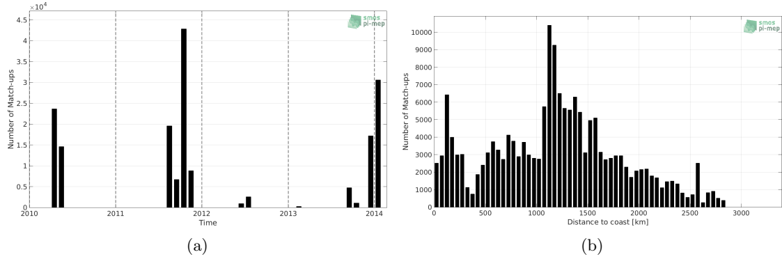
Figure 1: Number of match-ups between TSG-SAMOS and SMOS-L3-CATDS-CECOS-LOCEAN-V3-9DAYS-25KM SSS as a function of time (a) and as function of the distance to coast (b) over the South Atlantic Ocean Pi-MEP region and for the full satellite product period.
