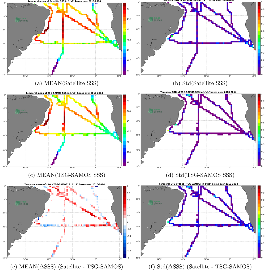
Figure 6: Temporal mean (left) and Std (right) of SSS from SMOS-L3-CATDS-CECOS-LOCEAN-V3-9DAYS-25KM (top), TSG-SAMOS (middle), and of \Delta SSS (Satellite - TSG-SAMOS). Only match-up pairs are used to generate these maps.
