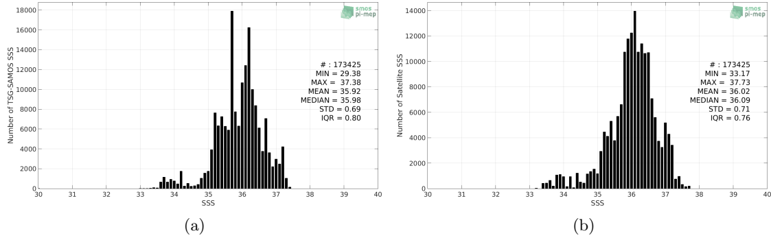
Figure 2: Histograms of SSS from TSG-SAMOS (a) and SMOS-L3-CATDS-CECOS-LOCEAN-V3-9DAYS-25KM (b) considering all match-up pairs per bins of 0.1 over the South Atlantic Ocean Pi-MEP region and for the full satellite product period.
