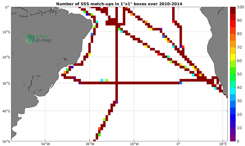
Figure 4: Number of SSS match-ups between TSG-SAMOS SSS and the SMOS-L3-CATDS-CECOS-LOCEAN-V3-9DAYS-25KM SSS product for the South Atlantic Ocean Pi-MEP region over 1^\circ \times 1^\circ boxes and for the full satellite product period.
