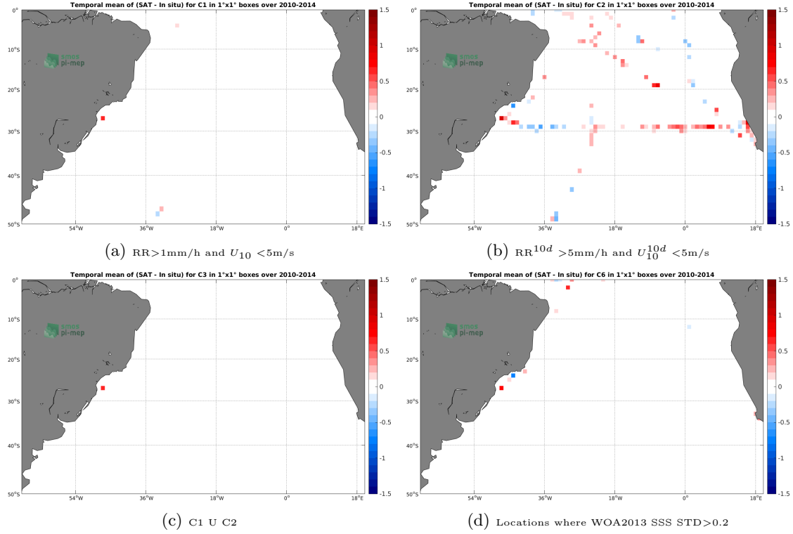
Figure 12: Temporal mean gridded over spatial boxes of size 1^\circ \times 1^\circ of \Delta SSS (SMOS-L3-CATDS-CECOS-LOCEAN-V3-9DAYS-25KM - TSG-SAMOS) for 4 different subdatasets corresponding to: RR > 1mm/h and U_{10} < 5\text{m/s} (a), RR^{10d} > 5\text{mm/h} and U_{10}^{10d} < 5\text{m/s} (b), C1 U C2 (c), Locations where WOA2013 SSS STD > 0.2 (d).
