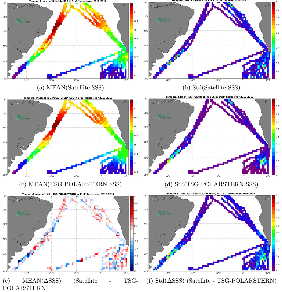
Figure 6: Temporal mean (left) and Std (right) of SSS from SMOS-L3-CATDS-CECOS-LOCEAN-V3-9DAYS-25KM (top), TSG-POLARSTERN (middle), and of \Delta SSS (Satellite - TSG-POLARSTERN). Only match-up pairs are used to generate these maps.
