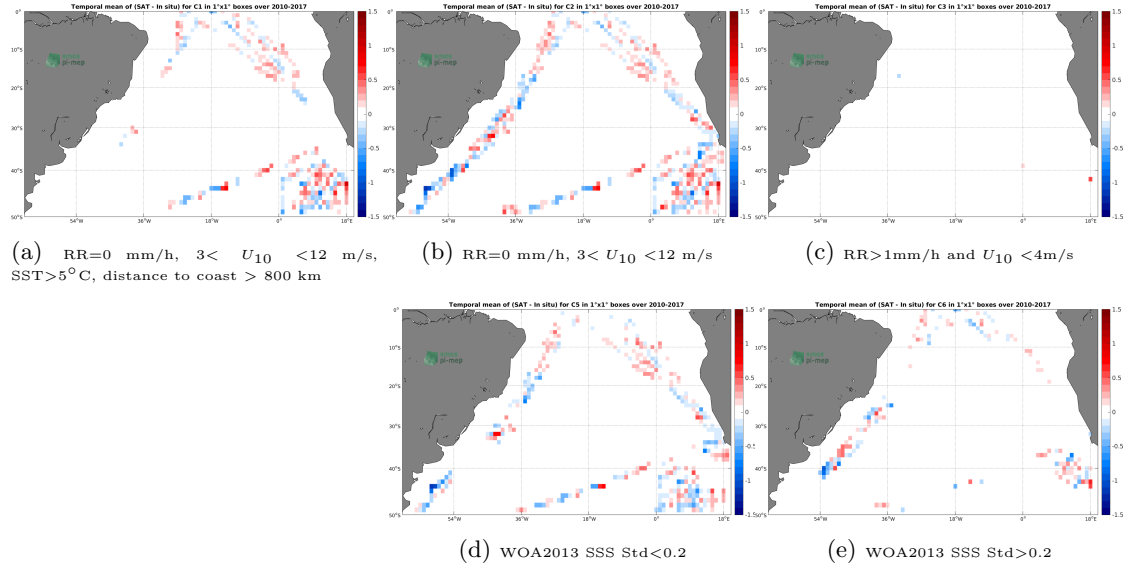
Figure 12: Temporal mean gridded over spatial boxes of size 1^\circ \times 1^\circ of \Delta SSS (SMOS-L3-CATDS-CECOS-LOCEAN-V3-9DAYS-25KM - TSG-POLARSTERN) for 5 different subdatasets corresponding to: RR=0 mm/h, 3 < U_{10} < 12 m/s, SST > 5^\circ C , distance to coast > 800 km (a), RR=0 mm/h, 3 < U_{10} < 12 m/s (b), RR > 1 mm/h and U_{10} < 4 m/s (c), WOA2013 SSS Std < 0.2 (d), WOA2013 SSS Std > 0.2 (e).
