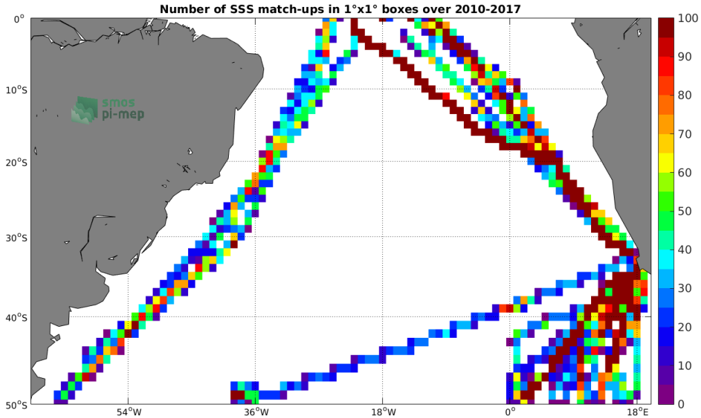
Figure 4: Number of SSS match-ups between TSG-POLARSTERN SSS and the SMOS-L3-CATDS-CECOS-LOCEAN-V3-9DAYS-25KM SSS product for the South Atlantic Ocean Pi-MEP region over 1^\circ \times 1^\circ boxes and for the full satellite product period.
