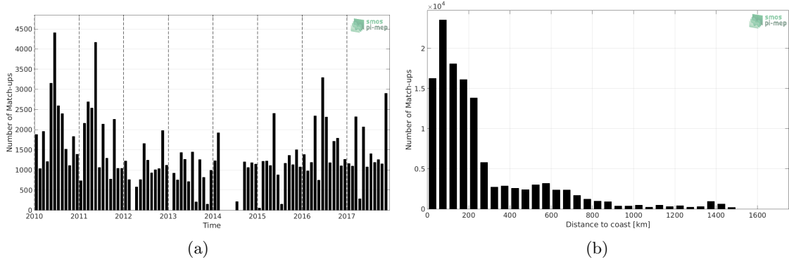
Figure 1: Number of match-ups between TSG-LEGOS-DM and SMOS-L3-CATDS-CECOS-LOCEAN-V3-9DAYS-25KM SSS as a function of time (a) and as function of the distance to coast (b) over the South Atlantic Ocean Pi-MEP region and for the full satellite product period.
