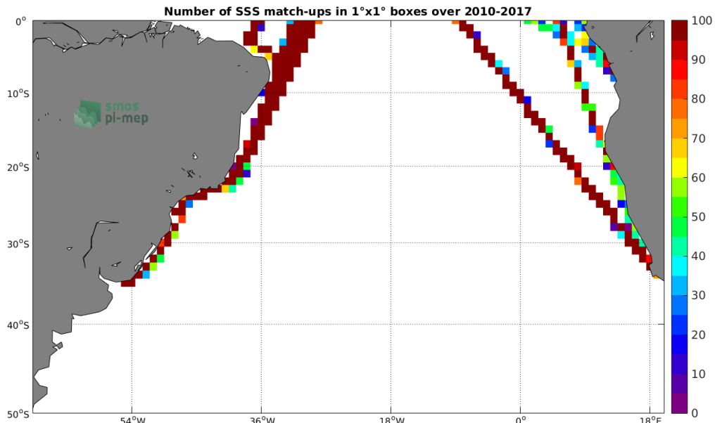
Figure 4: Number of SSS match-ups between TSG-LEGOS-DM SSS and the SMOS-L3-CATDS-CECOS-LOCEAN-V3-9DAYS-25KM SSS product for the South Atlantic Ocean Pi-MEP region over 1°x1° boxes and for the full satellite product period.
