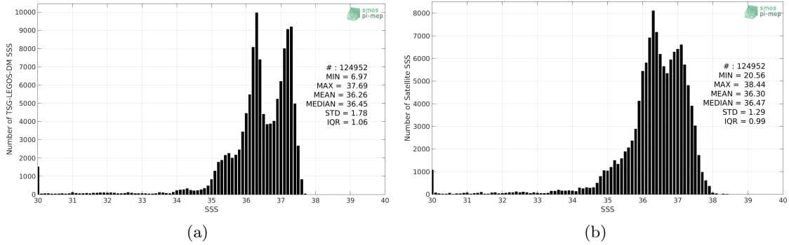
Figure 2: Histograms of SSS from TSG-LEGOS-DM (a) and SMOS-L3-CATDS-CECOS-LOCEAN-V3-9DAYS-25KM (b) considering all match-up pairs per bins of 0.1 over the South Atlantic Ocean Pi-MEP region and for the full satellite product period.
